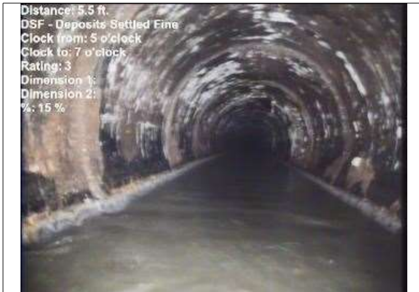
At: 5.5 ft. 5/7 DSF - Deposits Settled Fine Joint: No 15 %
