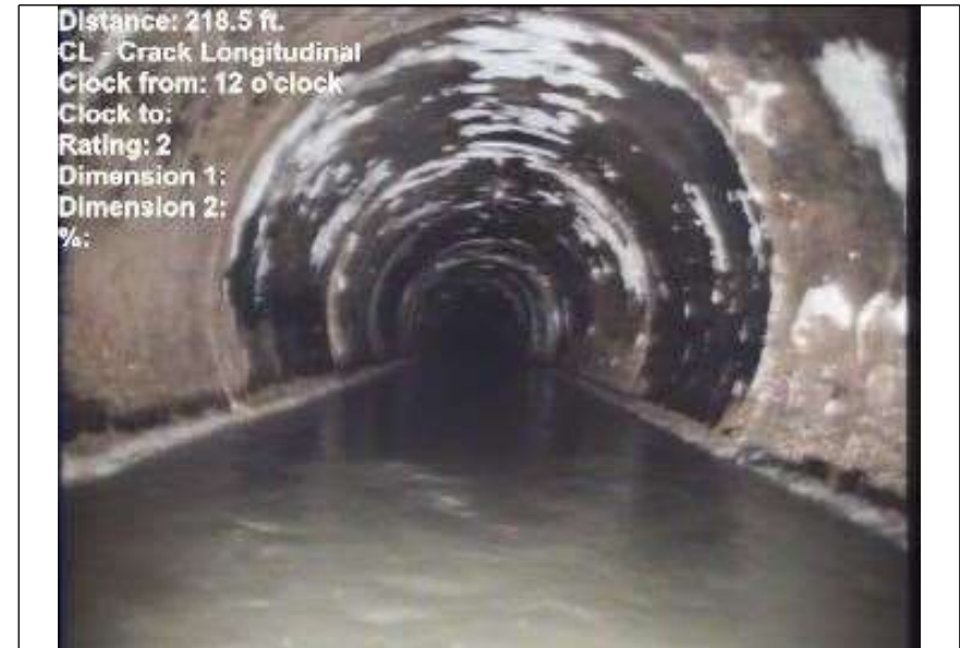
At: 218.5 ft. 12/. CL - Crack Longitudinal Joint: No
