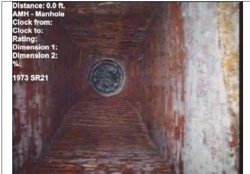
At: 0 ft. AMH - Manhole Joint: No 1973 SR21
