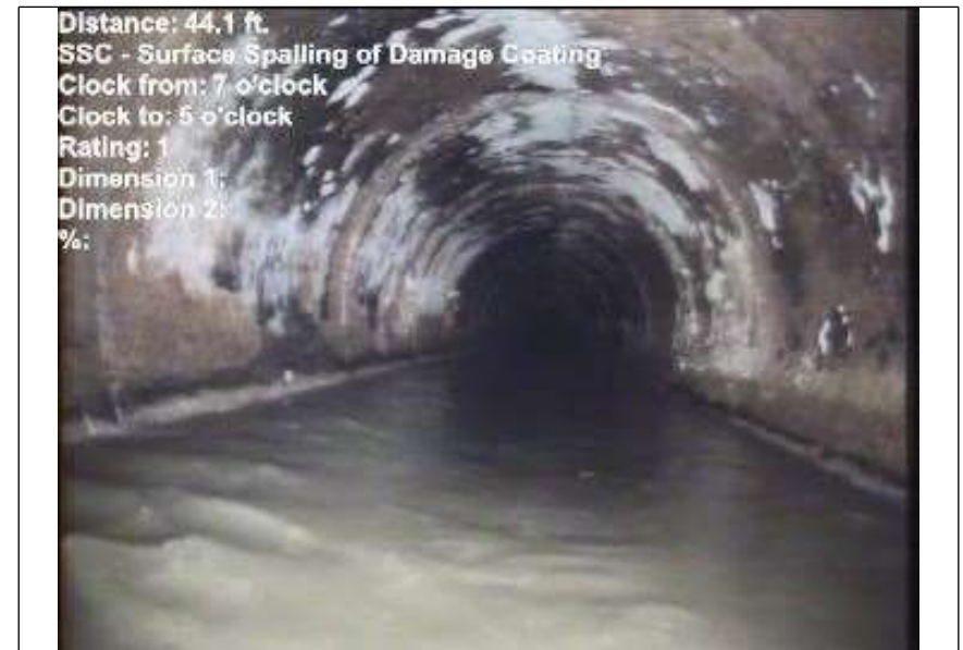
At: 44.1 ft. 7/5 SSC - Surface Spalling of Damage Coating Joint: No
