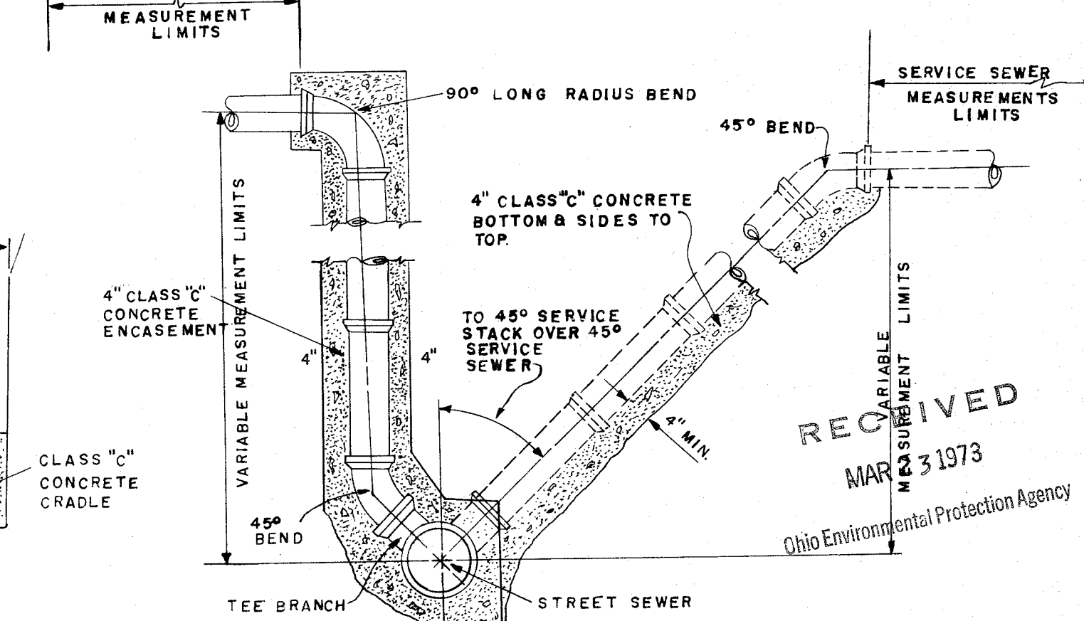
TYPICAL SERVICE STACK
