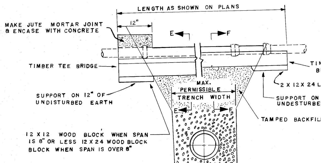
RESTORE EXIST. SEWER PIPE LINES
