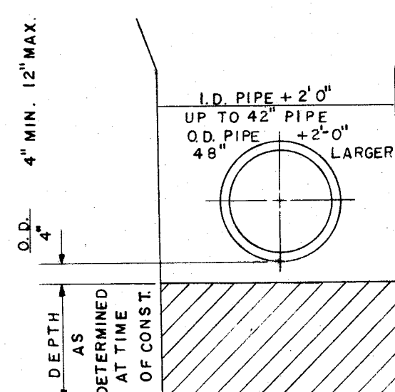
ADDITIONAL EARTH EXCAVATION PAYMENT LIMITS
