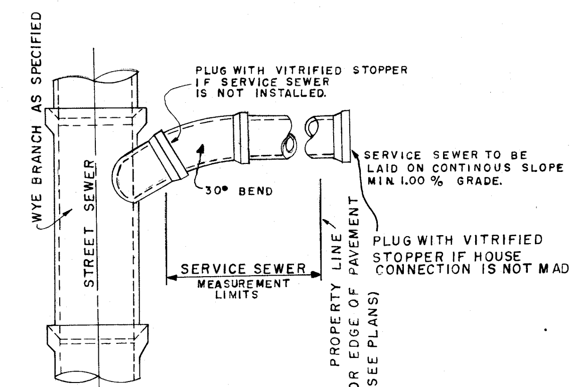
STANDARD SERVICE CONNECTION
