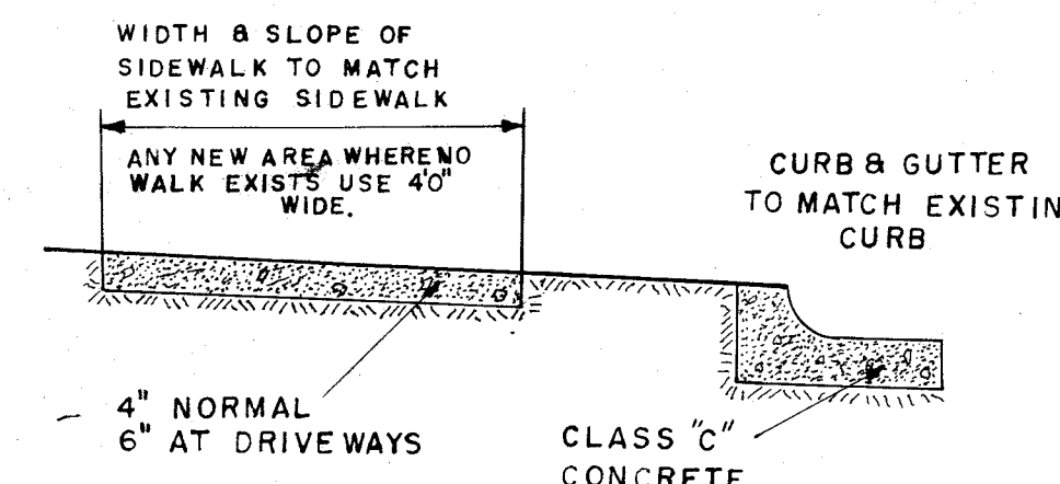
SIDEWALK CURB & GUTTER DETAIL
