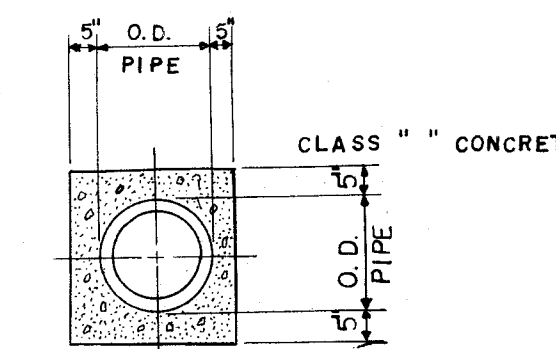
TYPICAL PIPE ENCASEMENT
