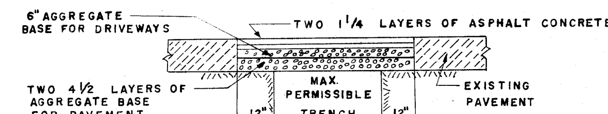
ASPHALT CONCRETE SURFACE COURSE AGGREGATE BASE COURSE
