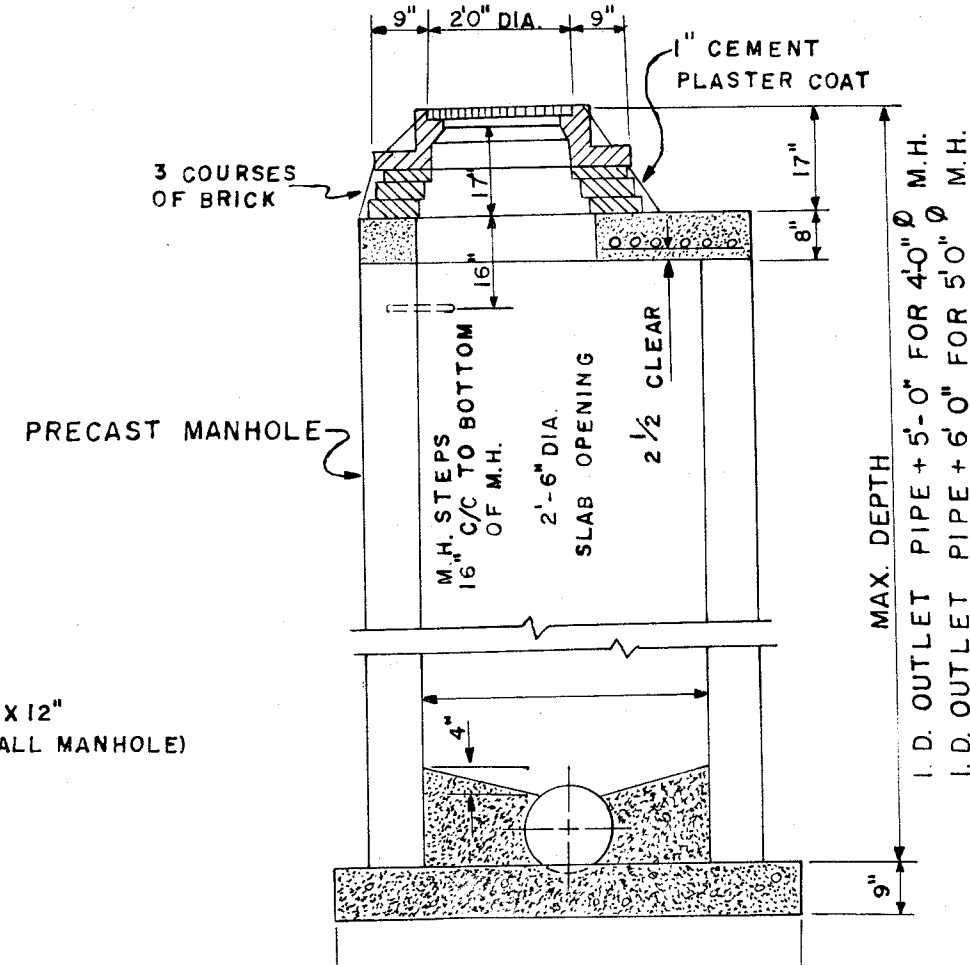
SECTION SHALLOW MANHOLE
