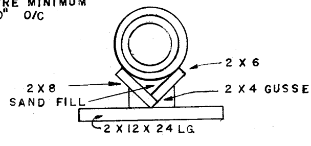
SECTION F-F
