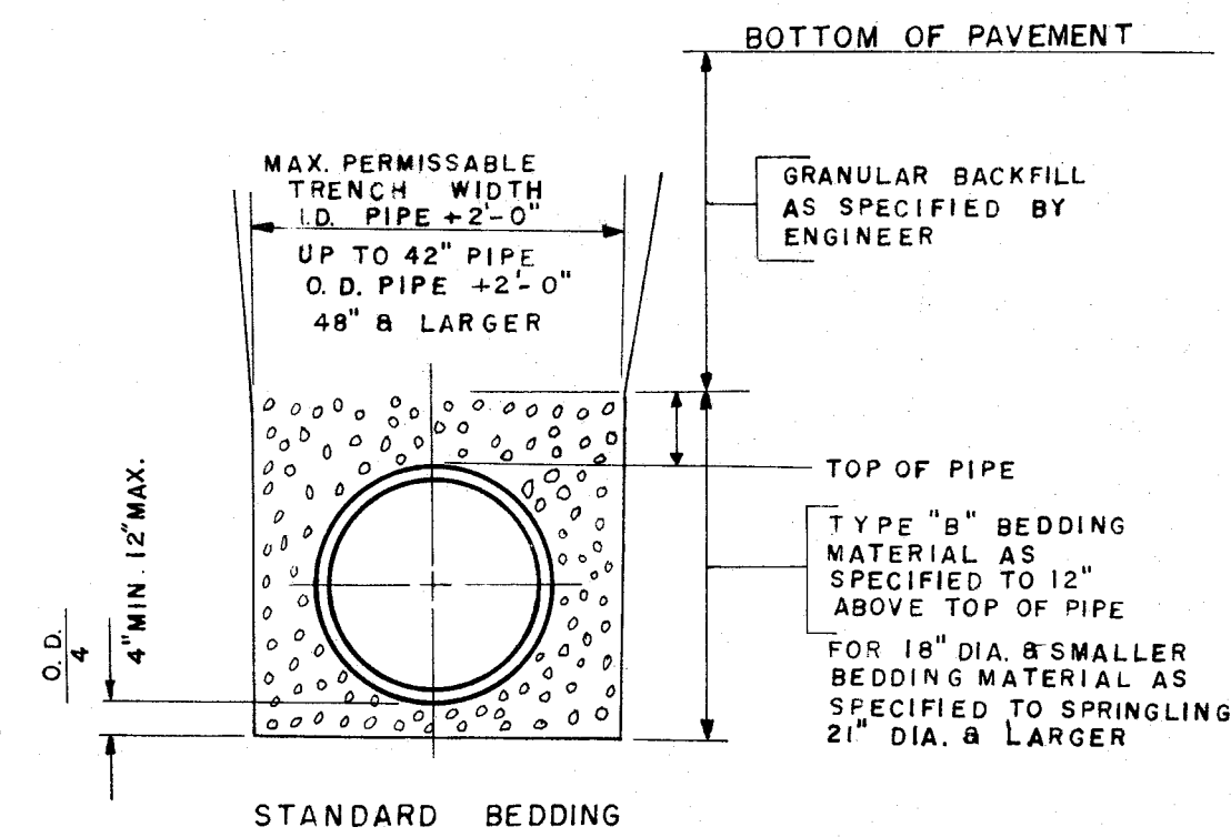
TYPE B BEDDING
