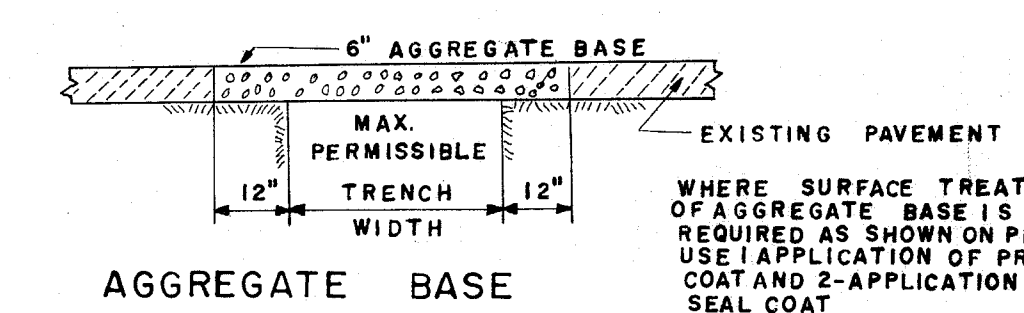
AGGREGATE BASE
