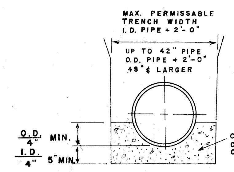
TYPE A BEDDING
