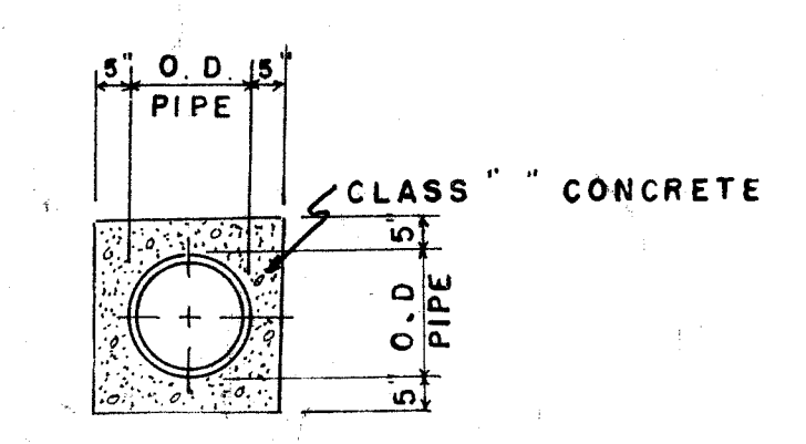
TYPICAL PIPE ENCASEMENT
