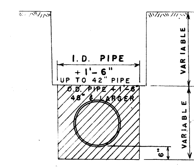
ROCK EXCAVATION PAYMENT LIMITS
