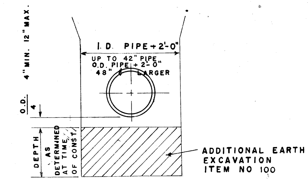
ADDITIONAL EARTH EXCAVATION PAYMENT LIMITS
