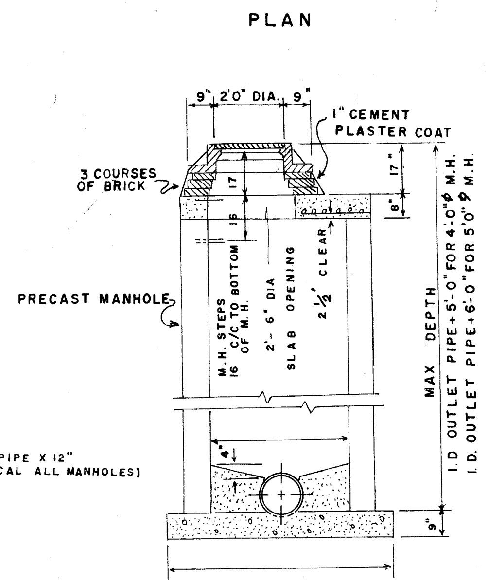
SECTION SHALLOW MANHOLE
