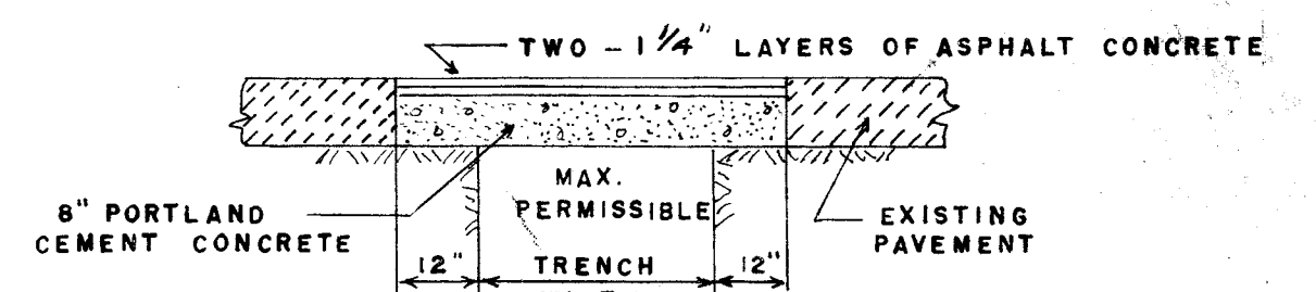
ASPHALT CONCRETE SURFACE COURSE PORTLAND CEMENT CONCRETE BASE COURSE
