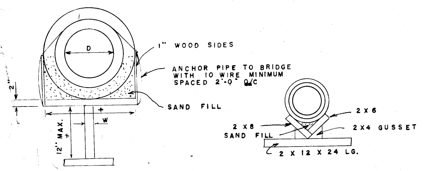
SECTION E-E
