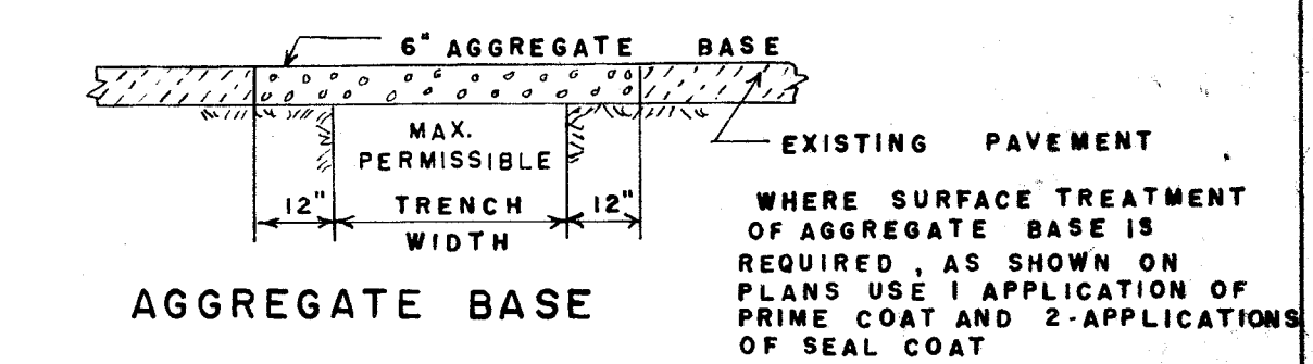
TYPICAL PAVEMENT REPLACEMENT SECTIONS
