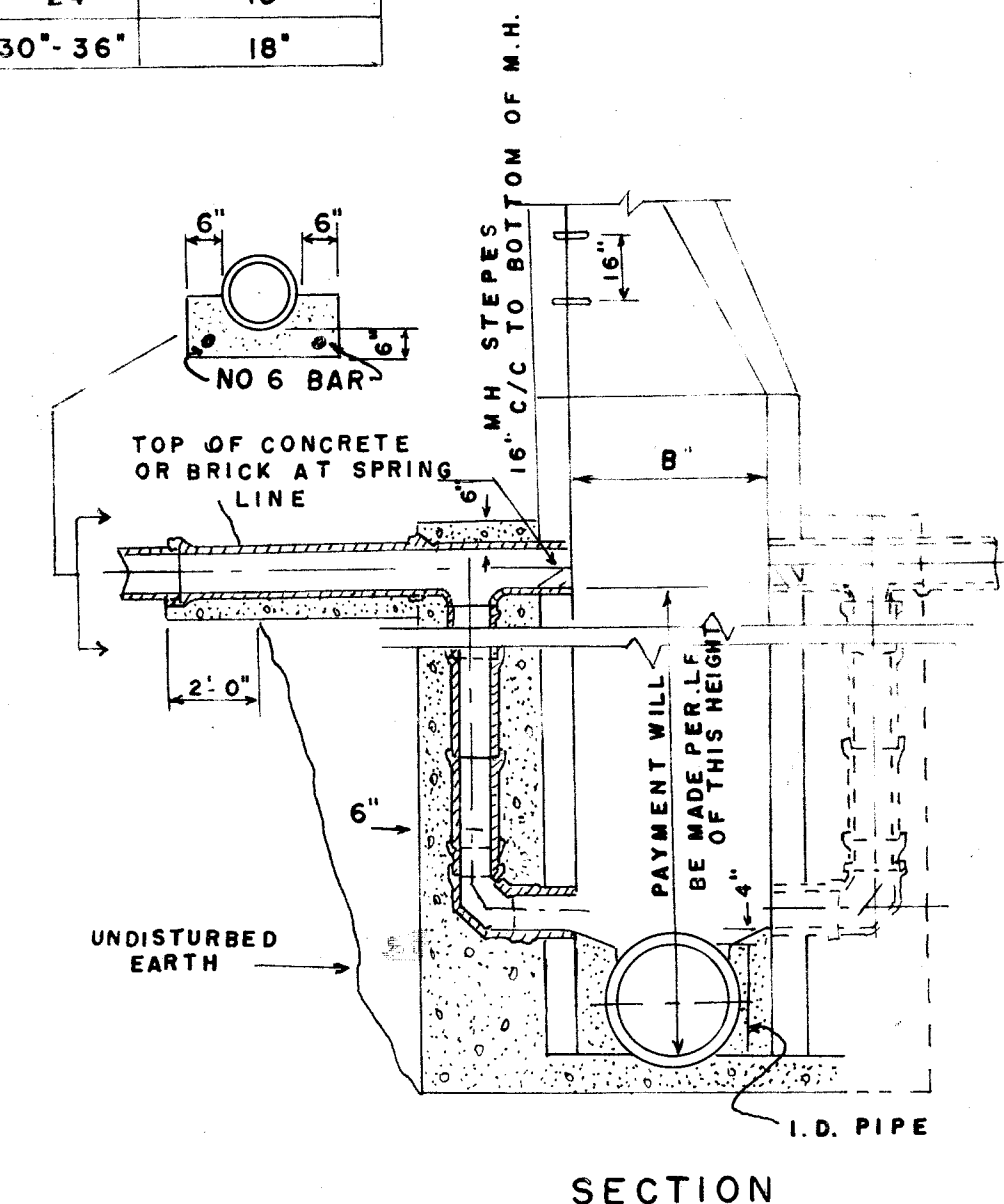
SECTION DROP MANHOLE
