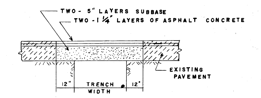
ASPHALT CONCRETE SURFACE COURSE SUB BASE
