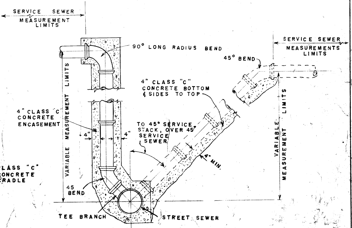
TYPICAL SERVICE STACK
