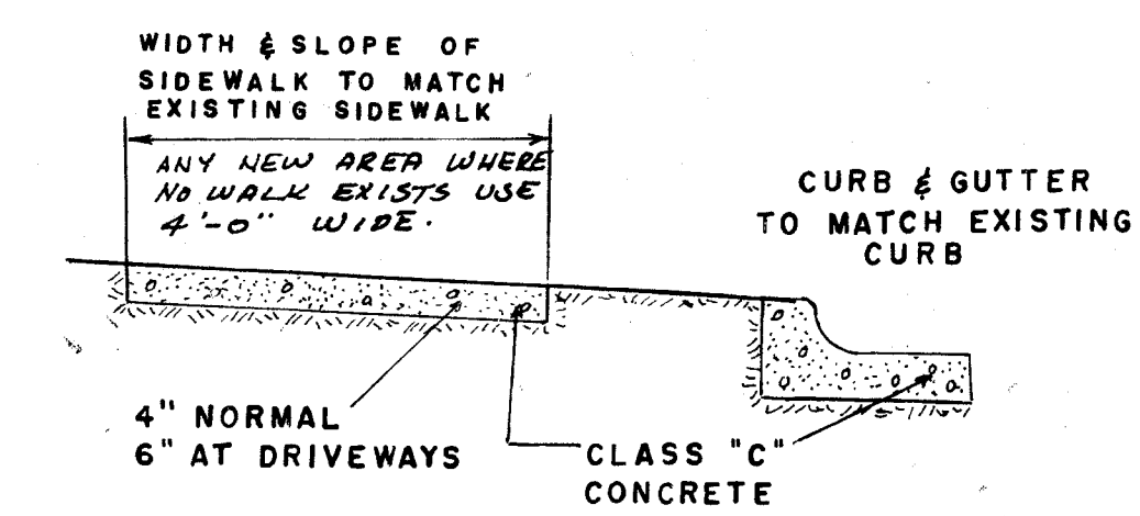
SIDEWALK CURB & GUTTER DETAIL
