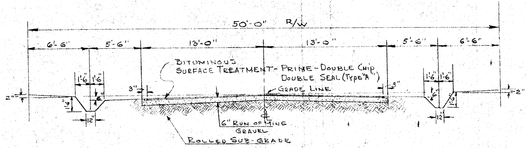
TYPICAL ROAD SECTION (TOWNSHIP)
