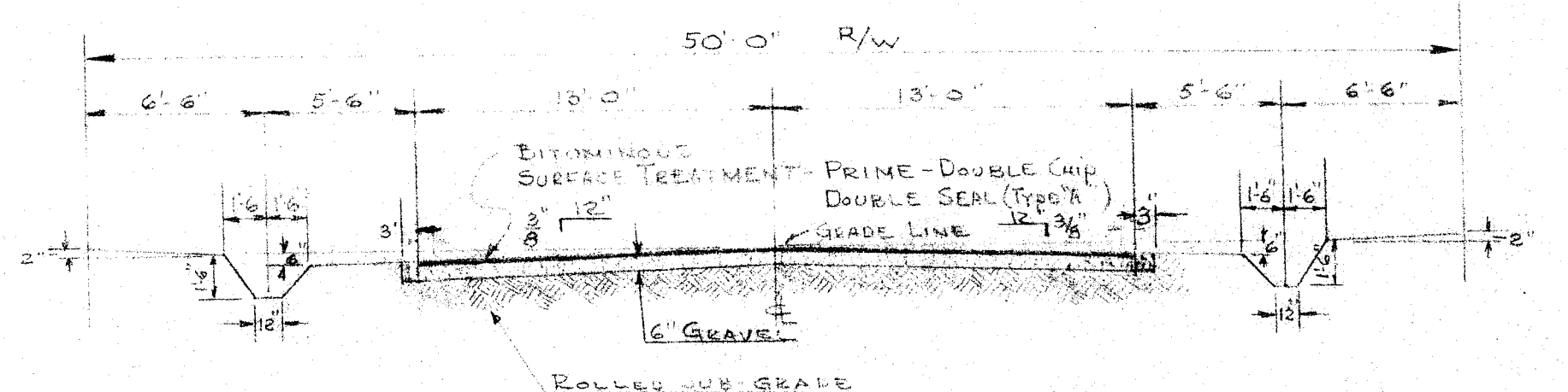
TYPICAL ROAD SECTION (TOWNSHIP)
