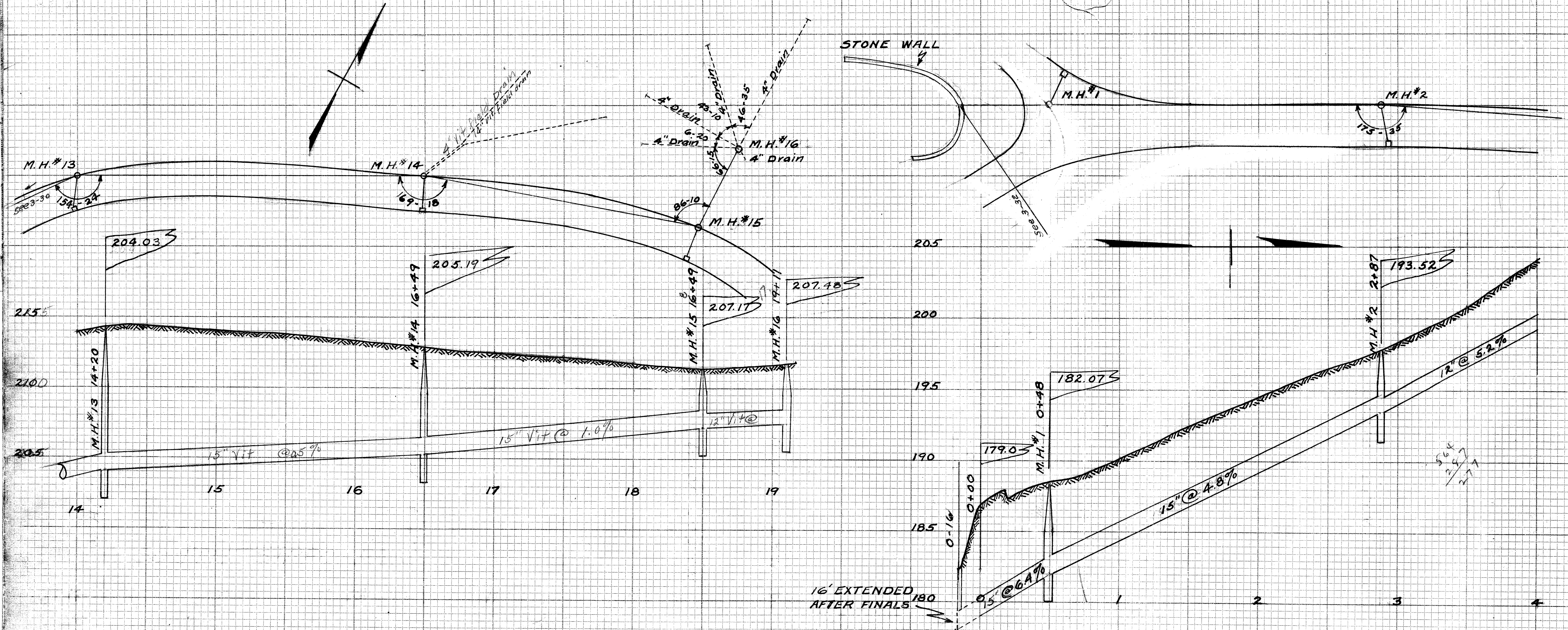
SOUTH SIPPO PARK STORM SEWER SYSTEM
