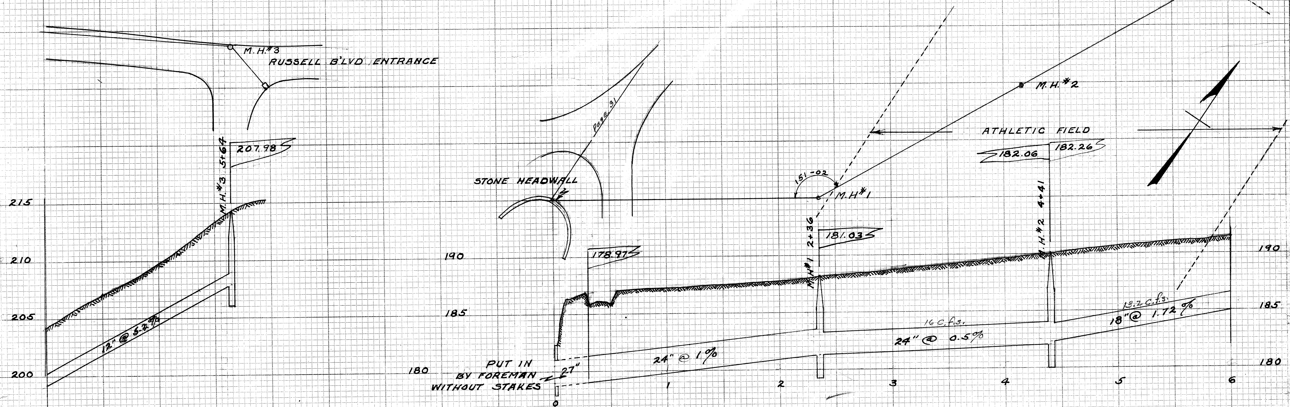
SOUTH SIPPO PARK STORM SEWER SYSTEM
