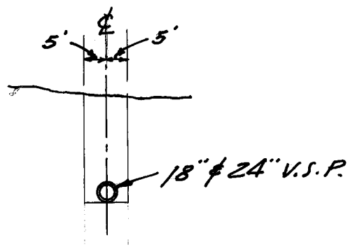
TYPICAL SECTION
