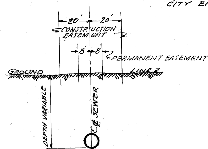
CROSS-SECTION
