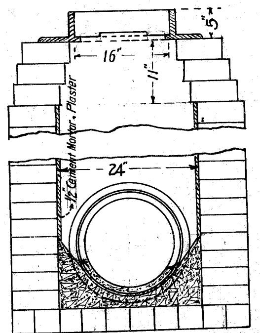
CROSS-SECTION OF INLET STYLE A
