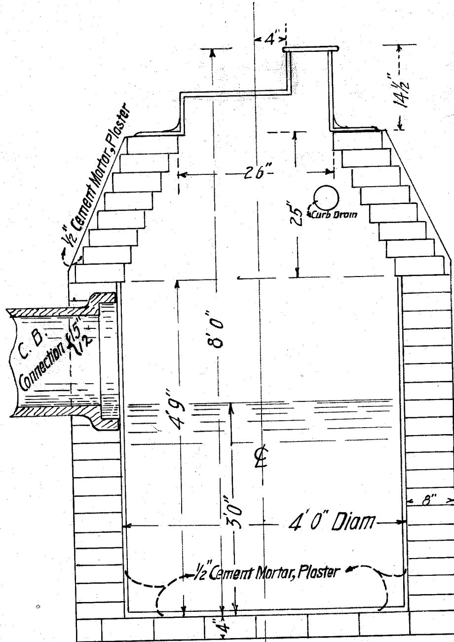
SECTION OF CATCH BASIN
