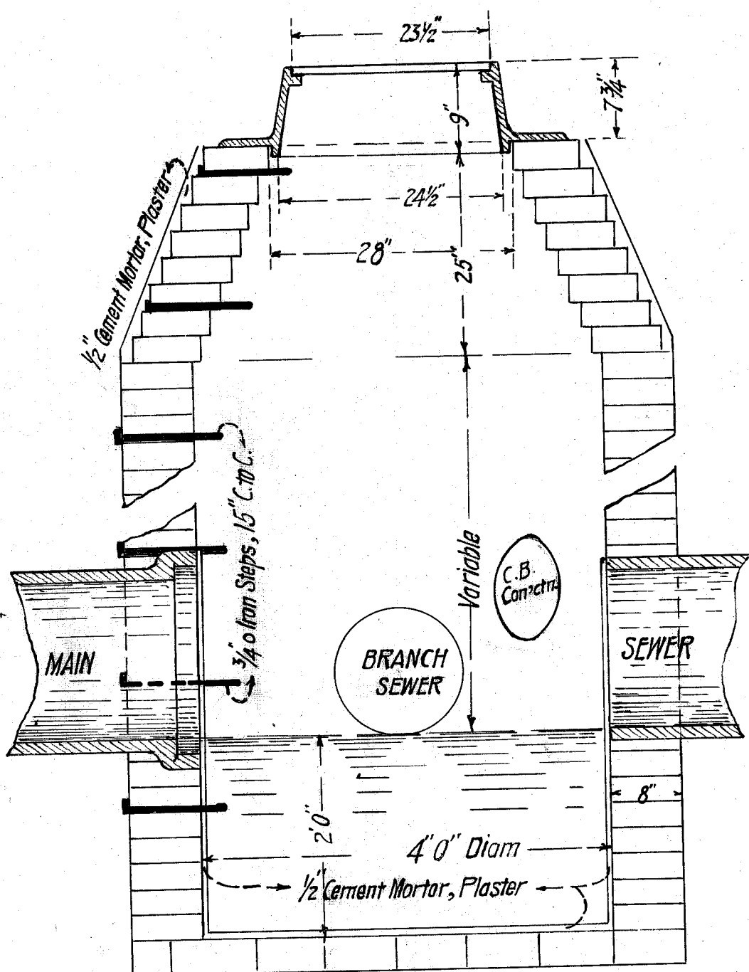
SECTION OF MANHOLE
