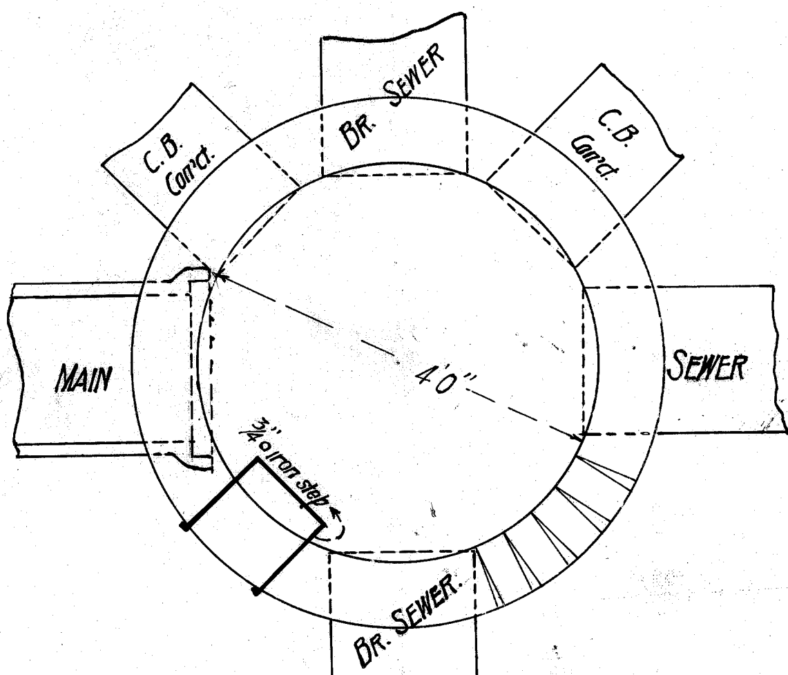
PLAN OF MANHOLE
