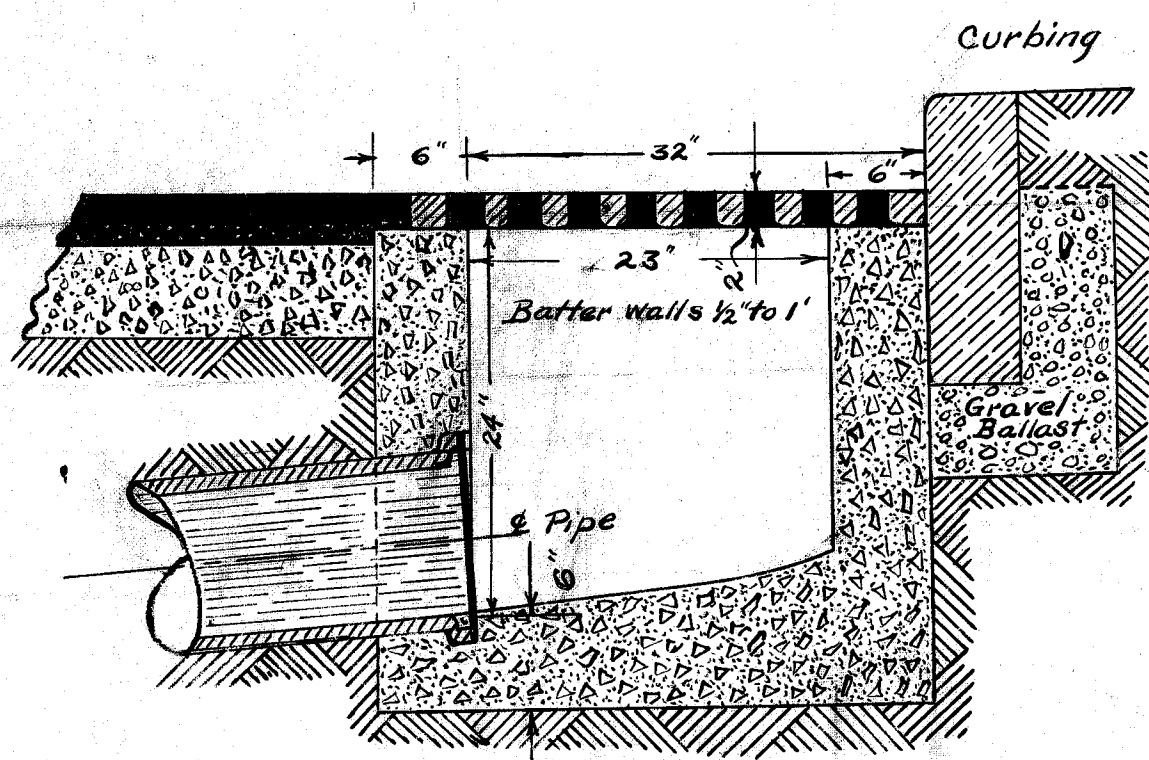
SECTIONAL VIEW (TRANSVERSE TO E P.V.M.T)
