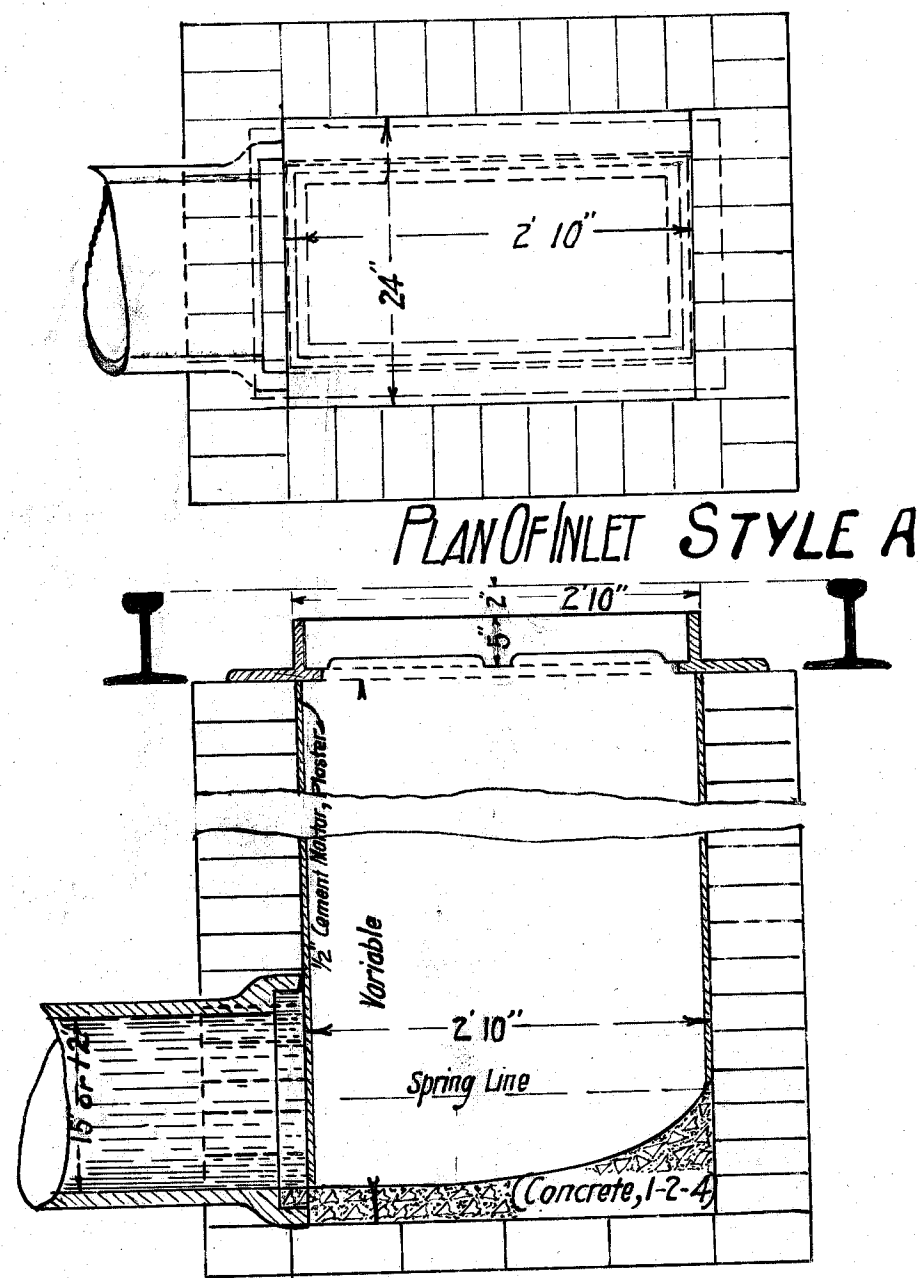
LONGITUDINAL SECTION OF INLET STYLE A
