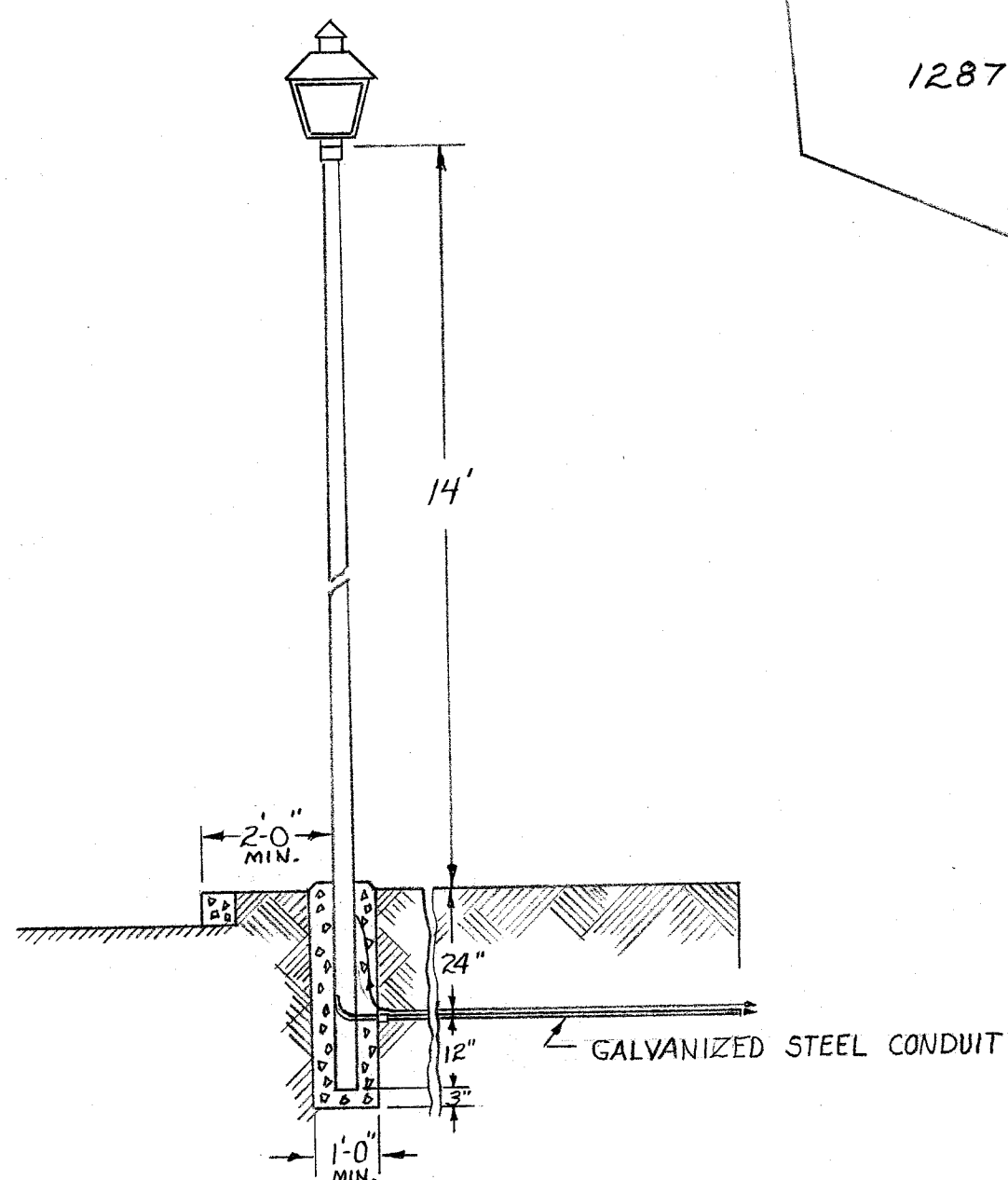
FOUNDATION DETAILS
