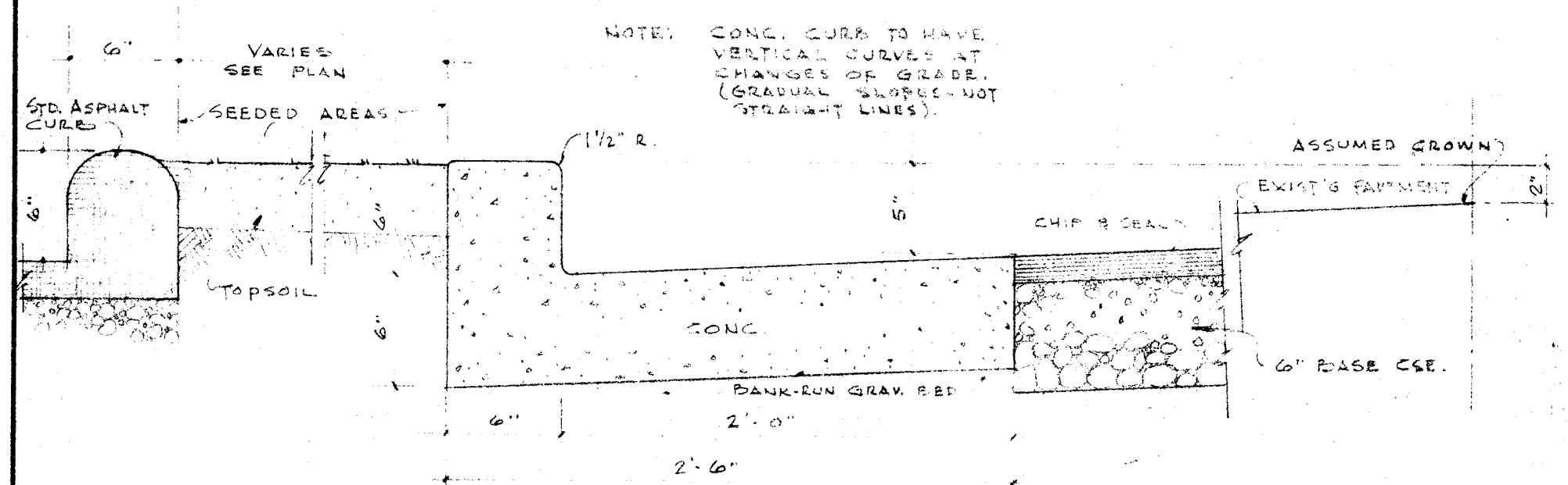
CURB & GUTTER DETAIL SCALE 1 1/2" = 1'-0"
