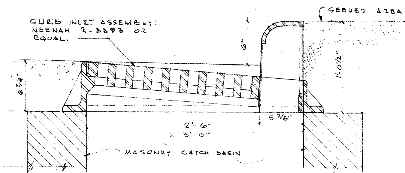
CURB-TYPE CATCH BASIN DETAIL CITY OF MASSILLON STANDARDS scale: 1-1/2" = 1'-0"
