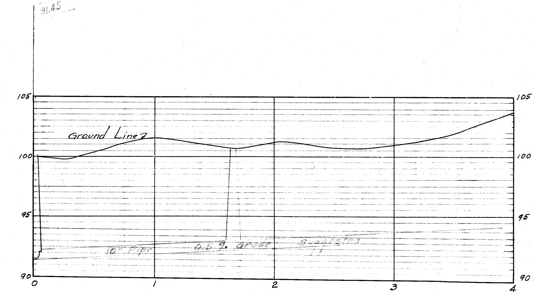
PROFILE OF PROPOSED SEWER
