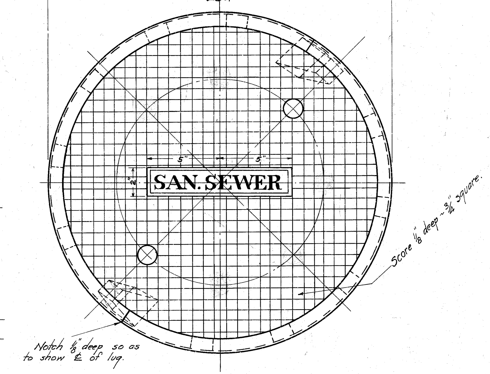
M.H. COVER TOP VIEW. WEIGHT 130 #
