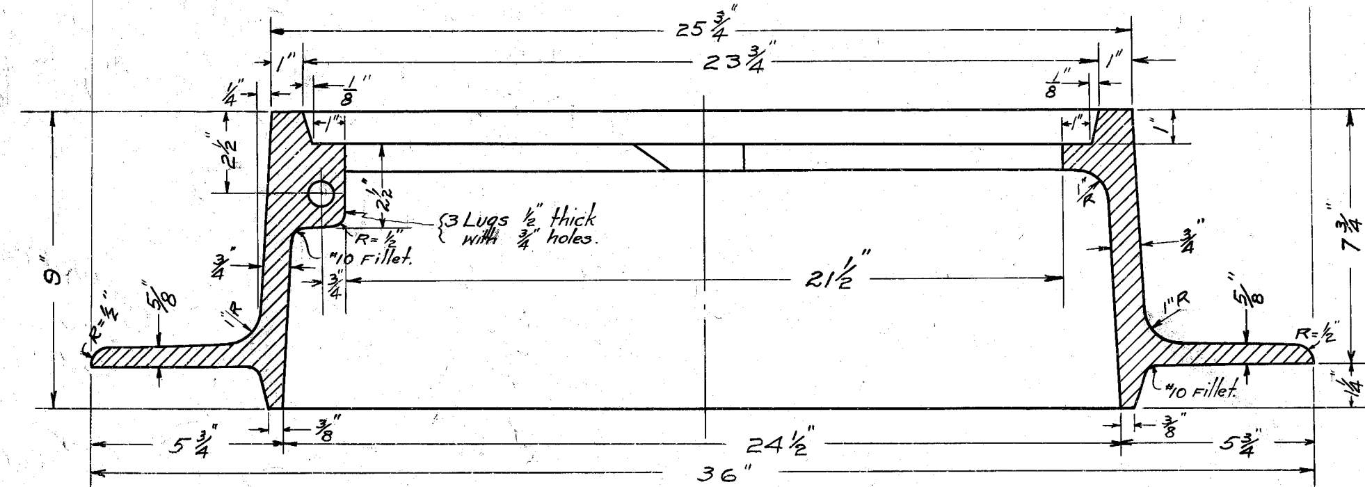
SECTION AT A-B. STANDARD PLAN WEIGHT 260 #
