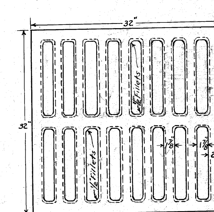
Top View TYPE B INLET CASTING - CAST IRON WEIGHT - 300 #
