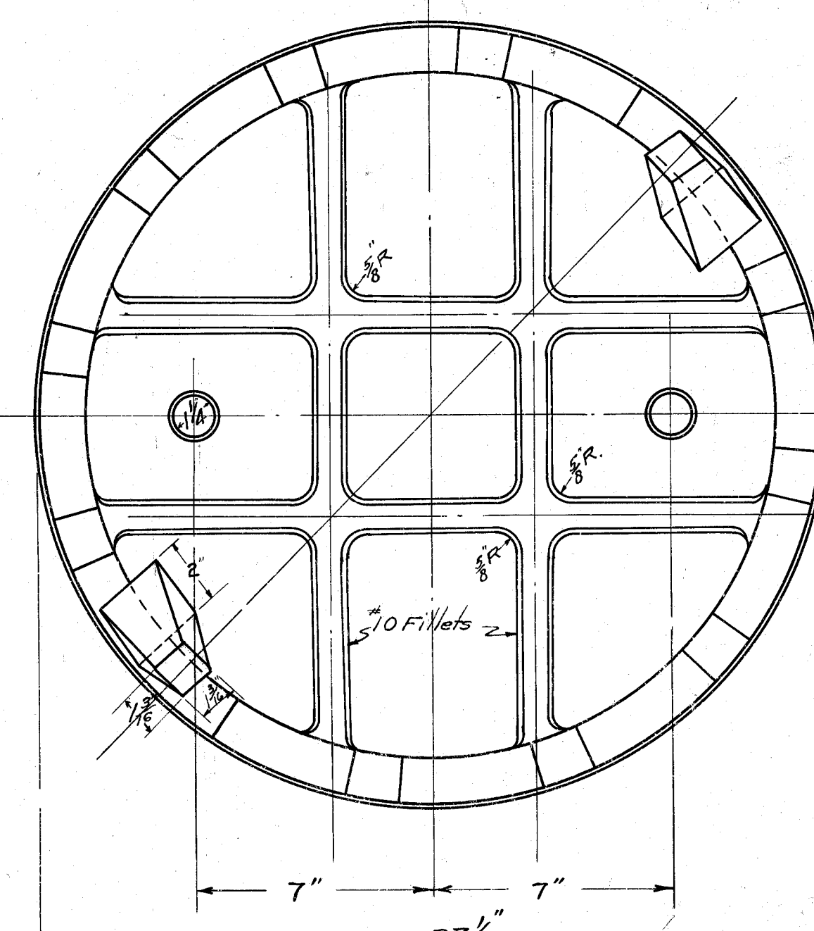
BOTTOM OF COVER FOR FL. TANKS.
