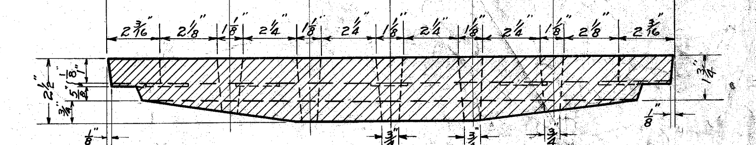
CROSS SECTION AT A-A. WEIGHT 112 #
