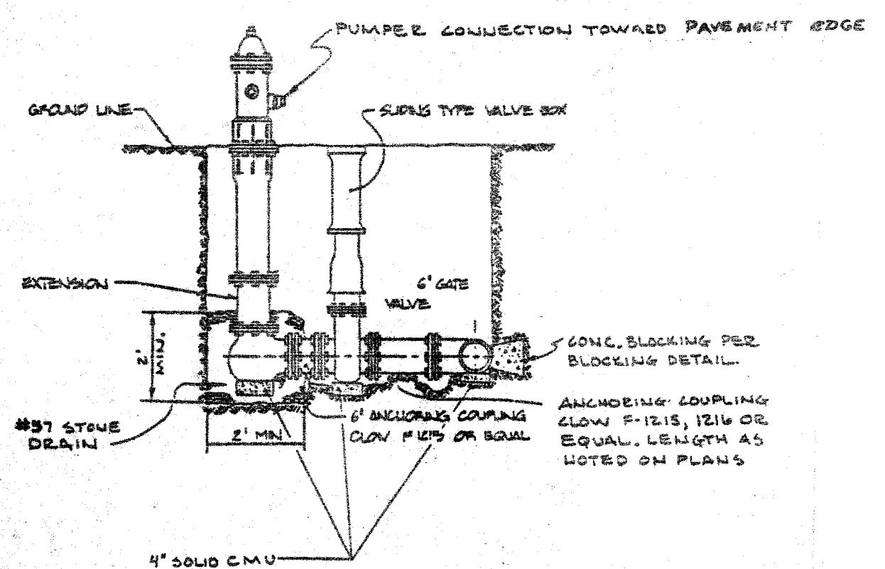
TYPICAL HYDRANT INSTALLATION PERPENDICULAR TO LINE
