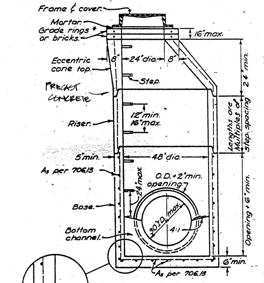
48" PRECAST BASE FOR 30" AND SMALLER PIPE PRECAST MANHOLE
