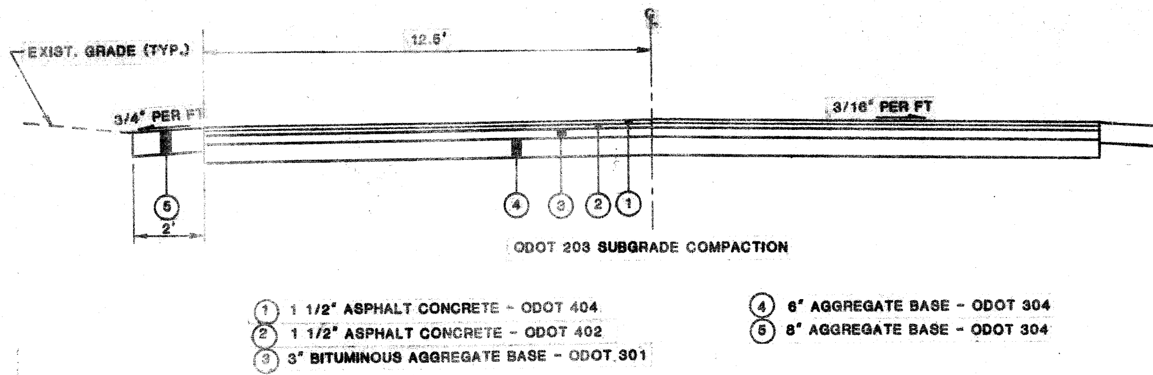
TYPICAL SECTION - ENTRANCE DRIVE DETAIL
