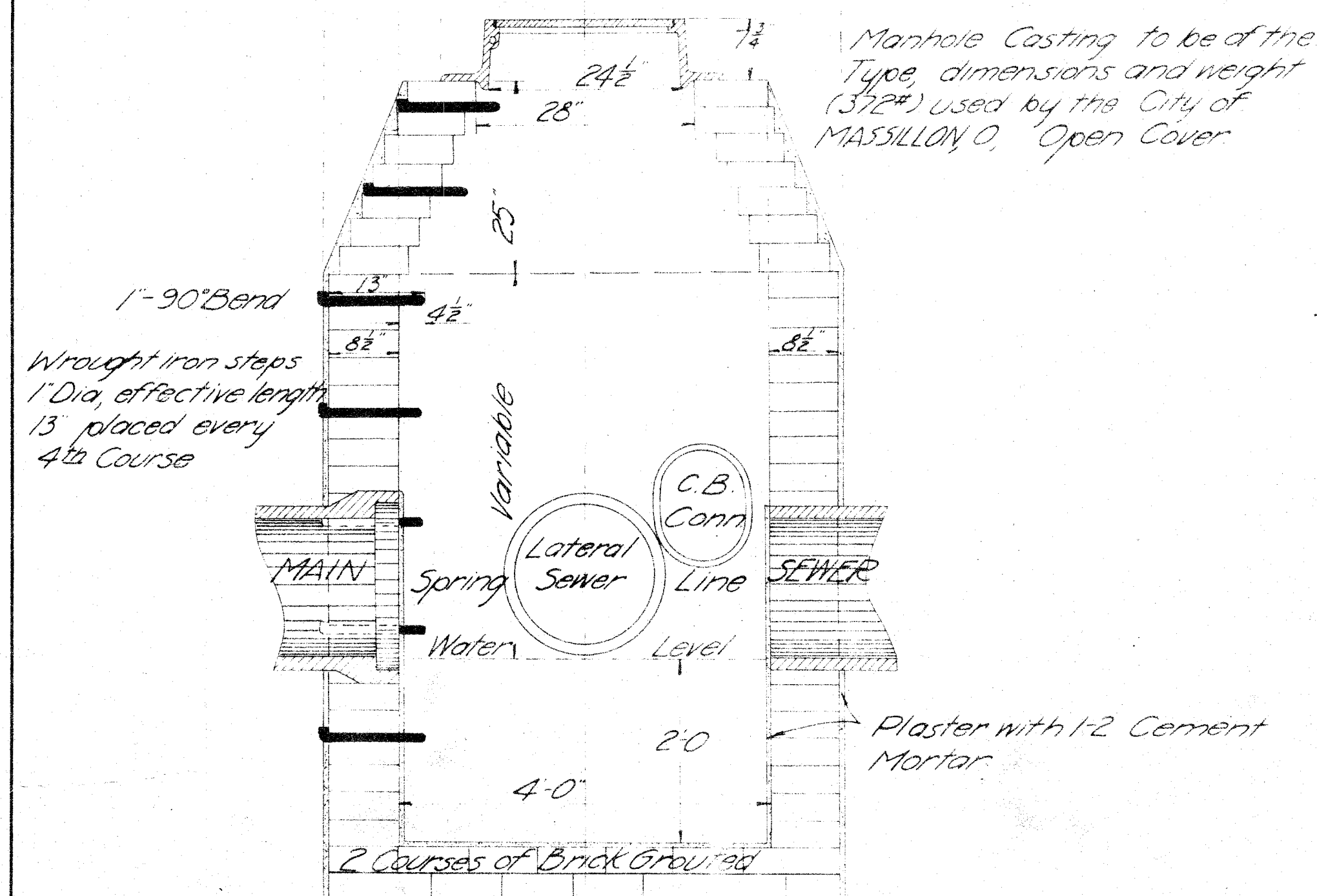
PLAN OF STANDARD MANHOLE FOR SECTION MASSILLON
