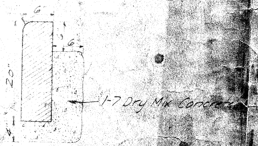
CROSS SECTION OF GRANITE CIRCLE CURB - SHOWING CONCRETE FOUNDATION AND BACKUP
