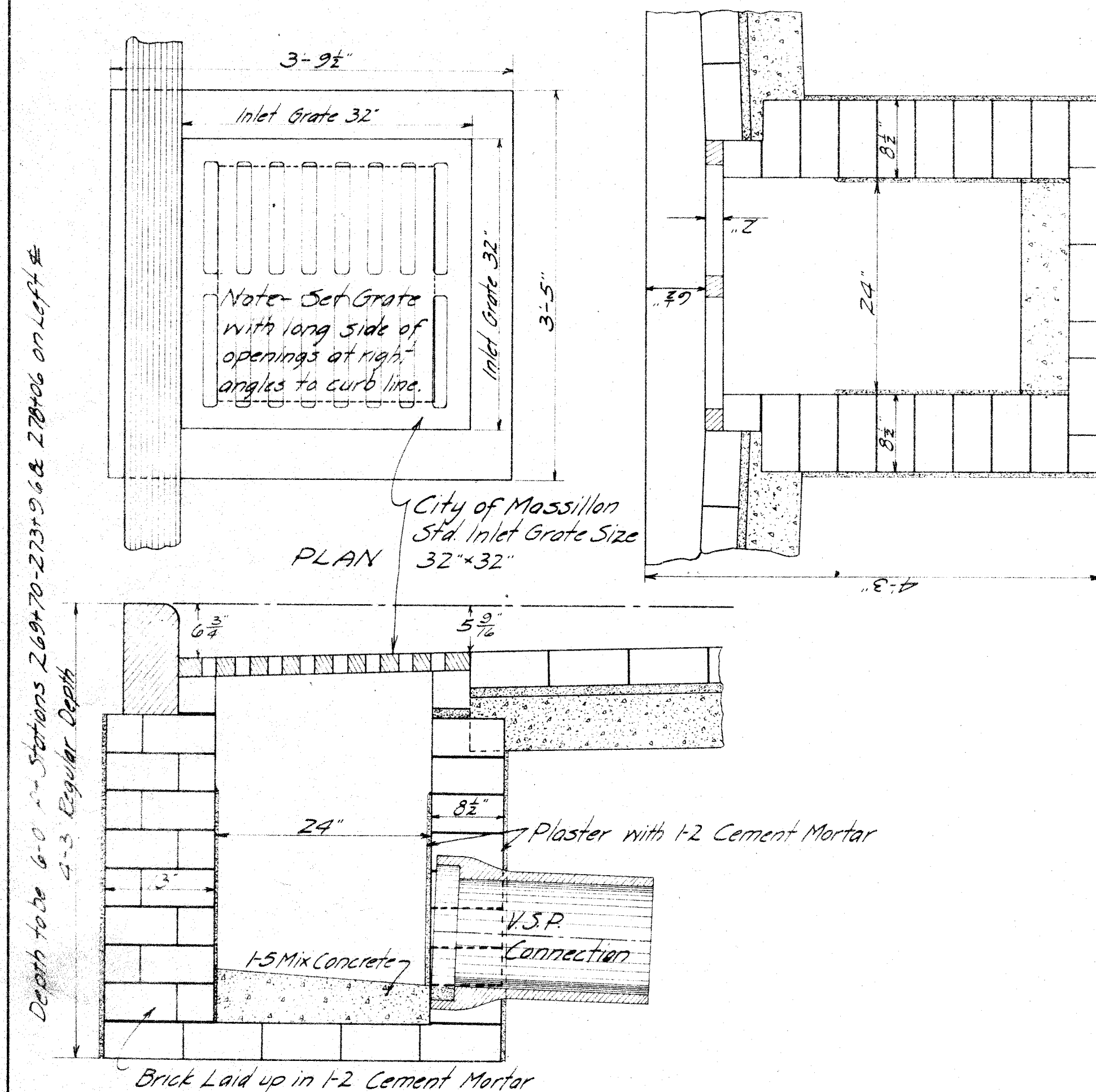
PLAN OF STORM WATER INLET FOR "SECTION MASSILLON" SEWERS
