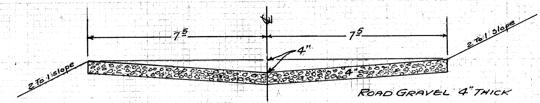
TYPICAL SECTION
