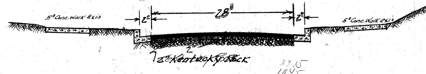
SECTIONAL VIEW 22+70 Lin. Ft.
