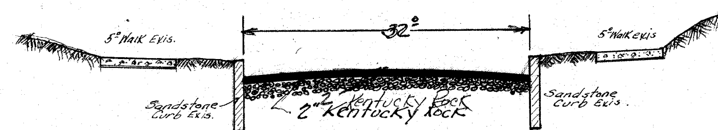
SECTIONAL VIEW 10+05 Lin. Ft.
