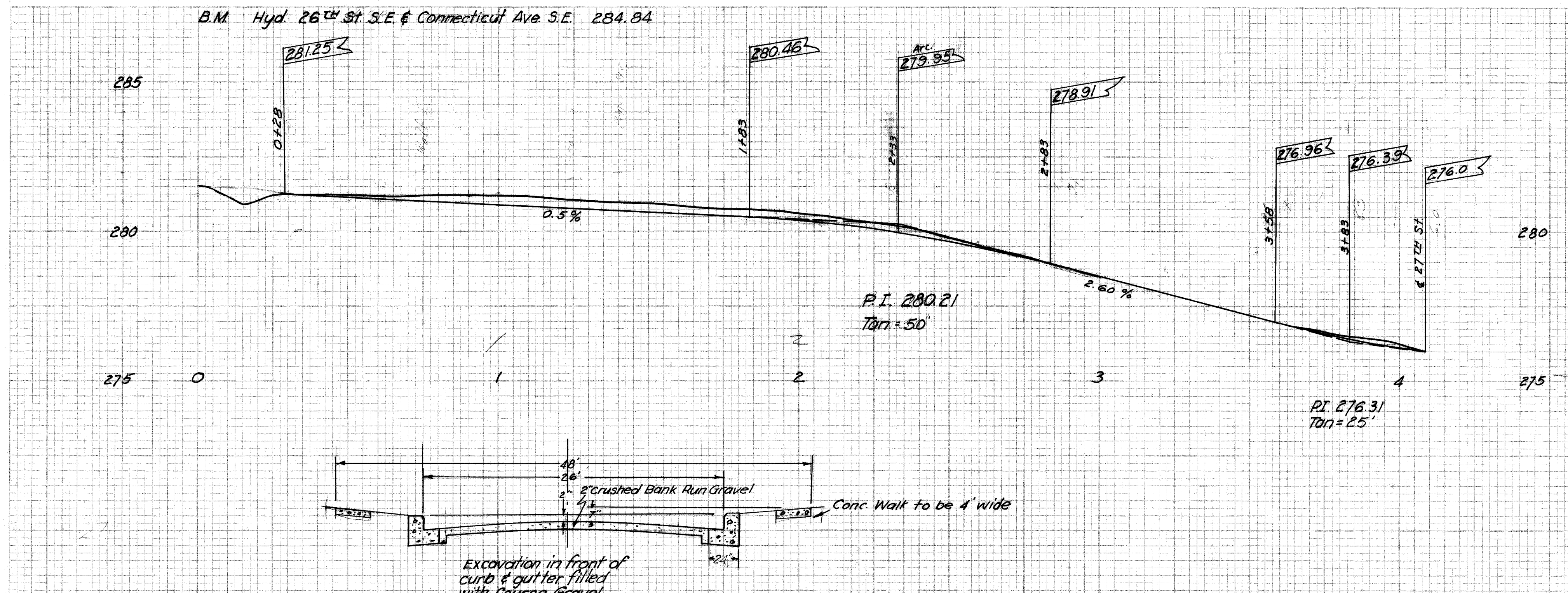
TYPICAL SECTION
