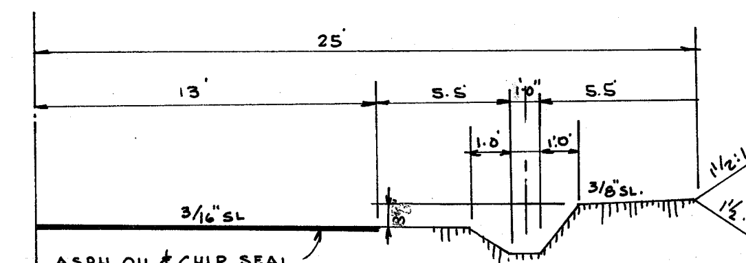
TYPICAL HALF SECTION:
