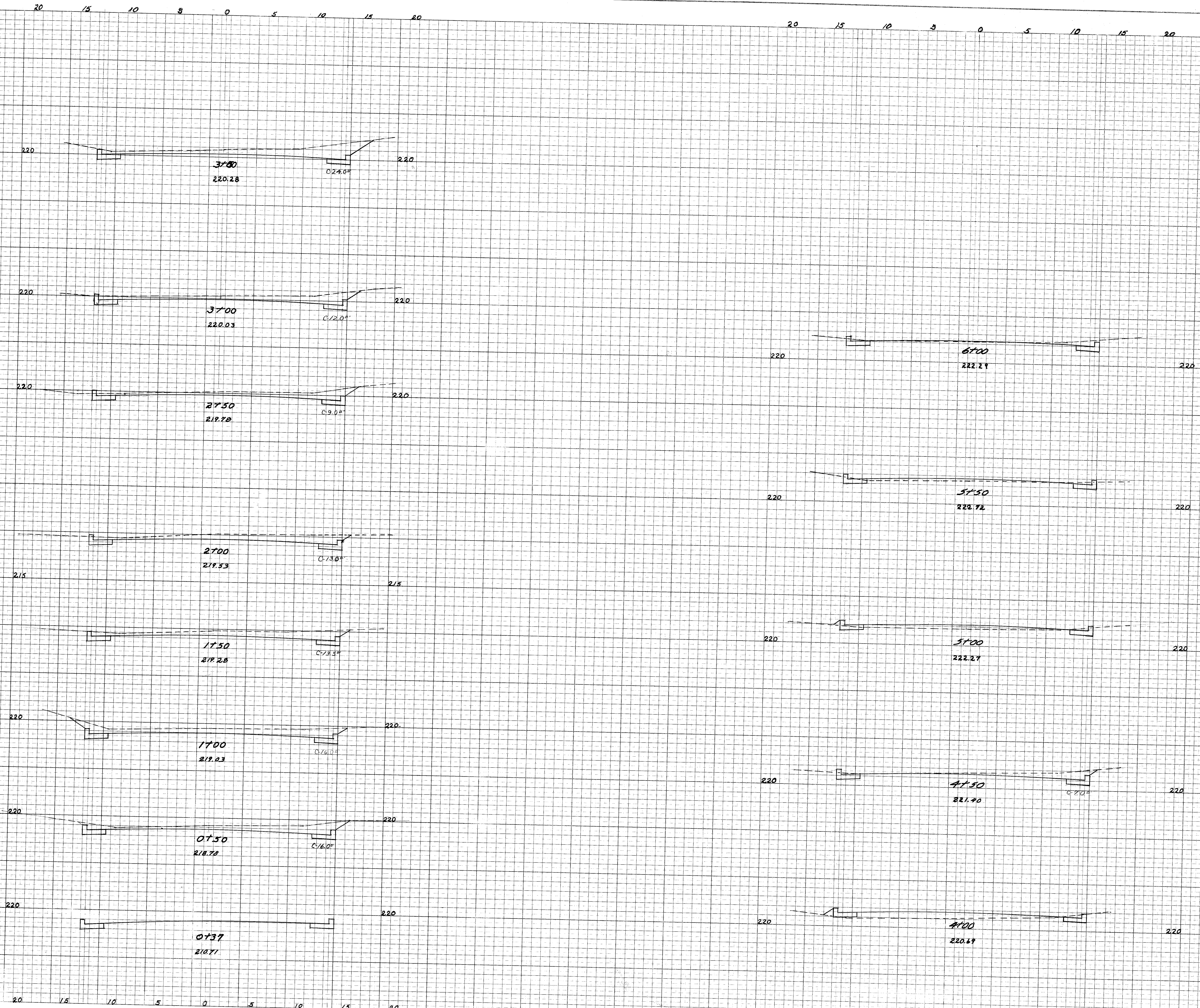
21 ST STREET NW CROSS SECTIONS
