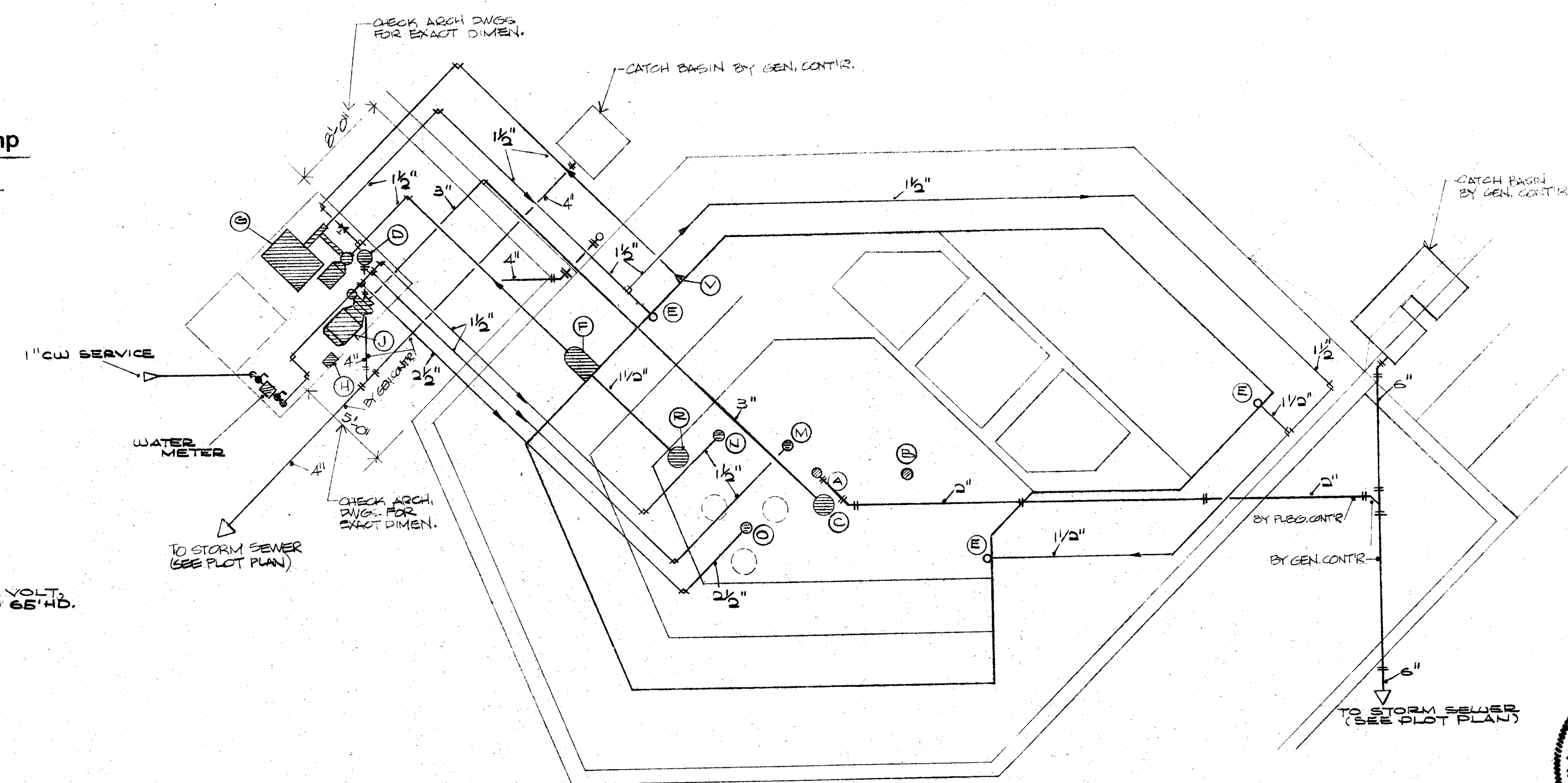
Fountain Plan SCALE 1/4" = 1'-0"
