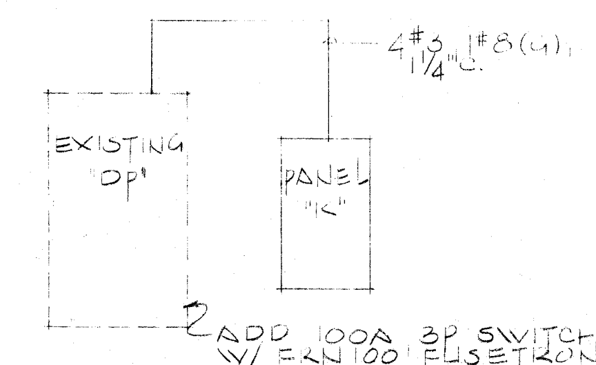
POWER RISER DIAGRAM NO SCALE
