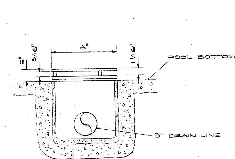
Main Sump For Circulating Pump NO SCALE
