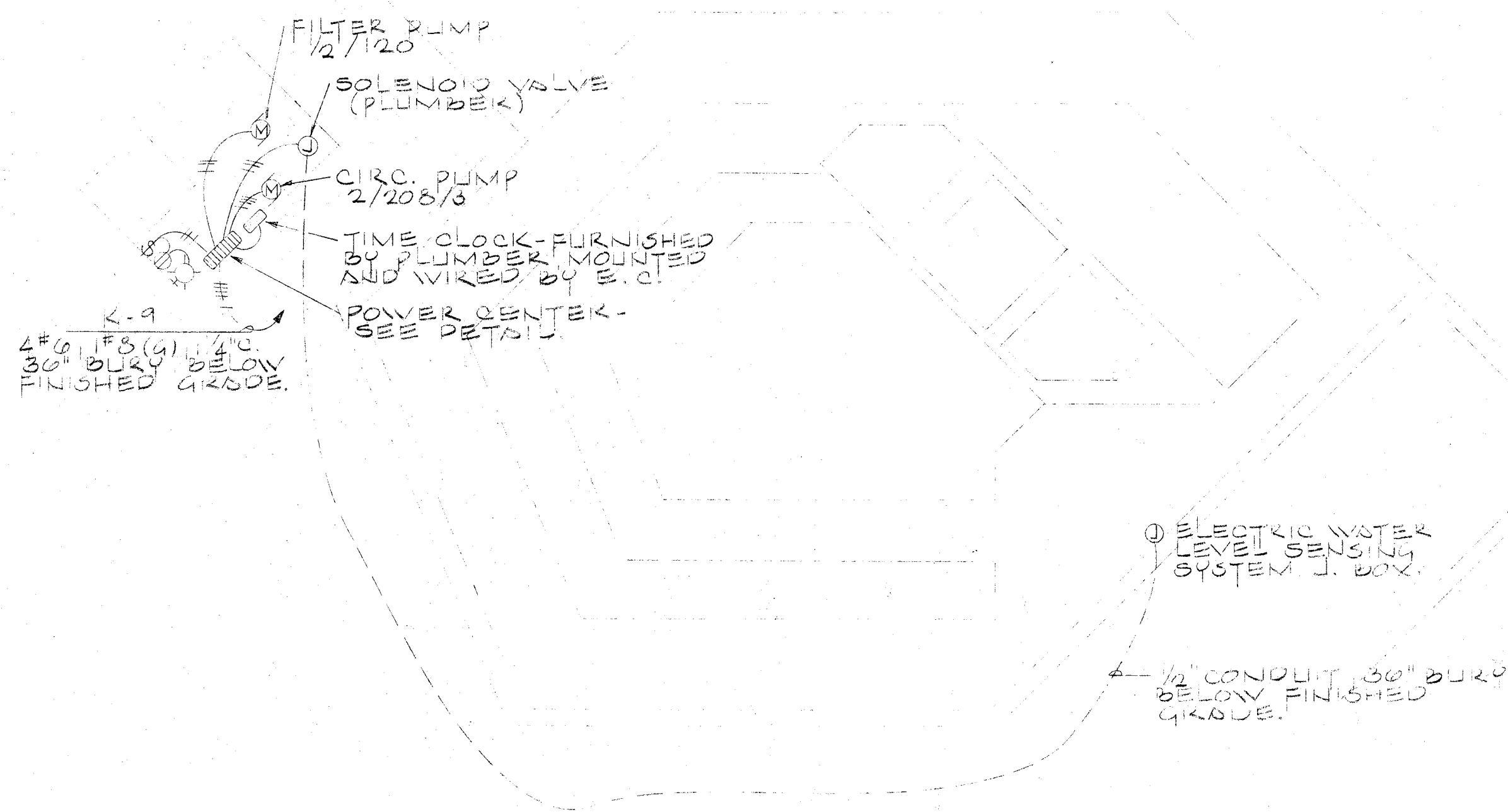
FOUNTAIN PLAN SCALE 1/4" = 1'-0"
