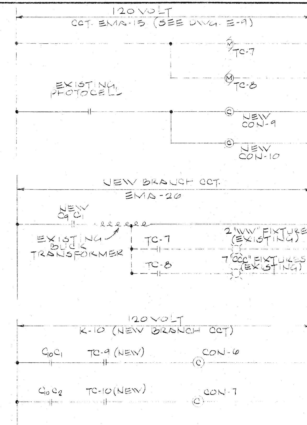
OUTSIDE LIGHTING CONTROL DIAGRAMS NO SCALE
