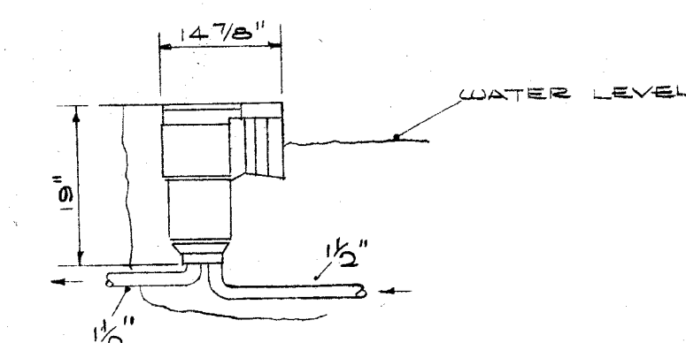
Surface Skimmer Filter System NO SCALE
