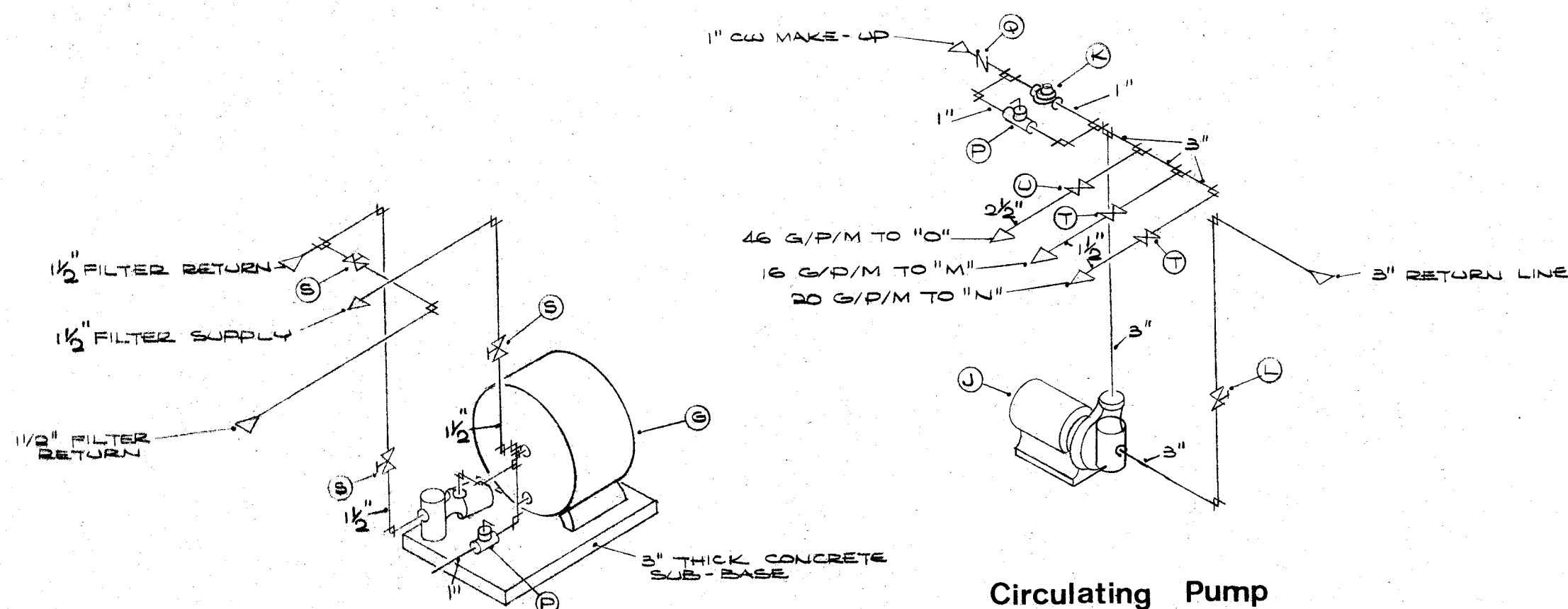
Circulating Pump Piping Detail NO SCALE
