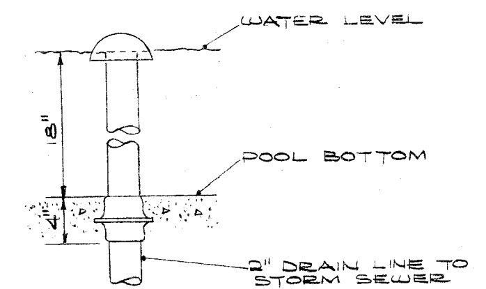
Overflow Drain NO SCALE
