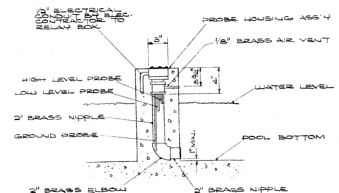
Electric Water Level Sensing System NO SCALE
