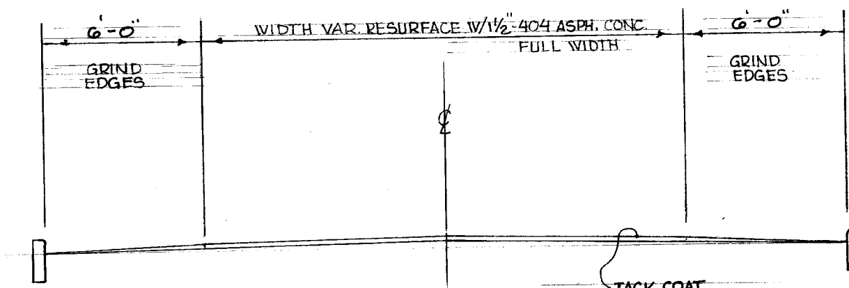
TYPICAL SECTION SCALE 1" = 5'
