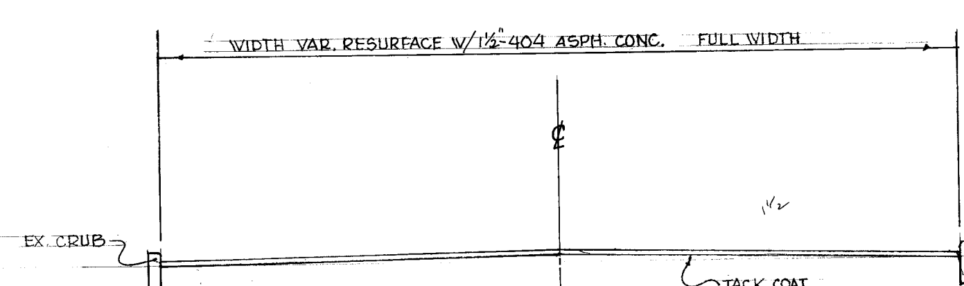
TYPICAL SECTION SCALE 1" = 5'
