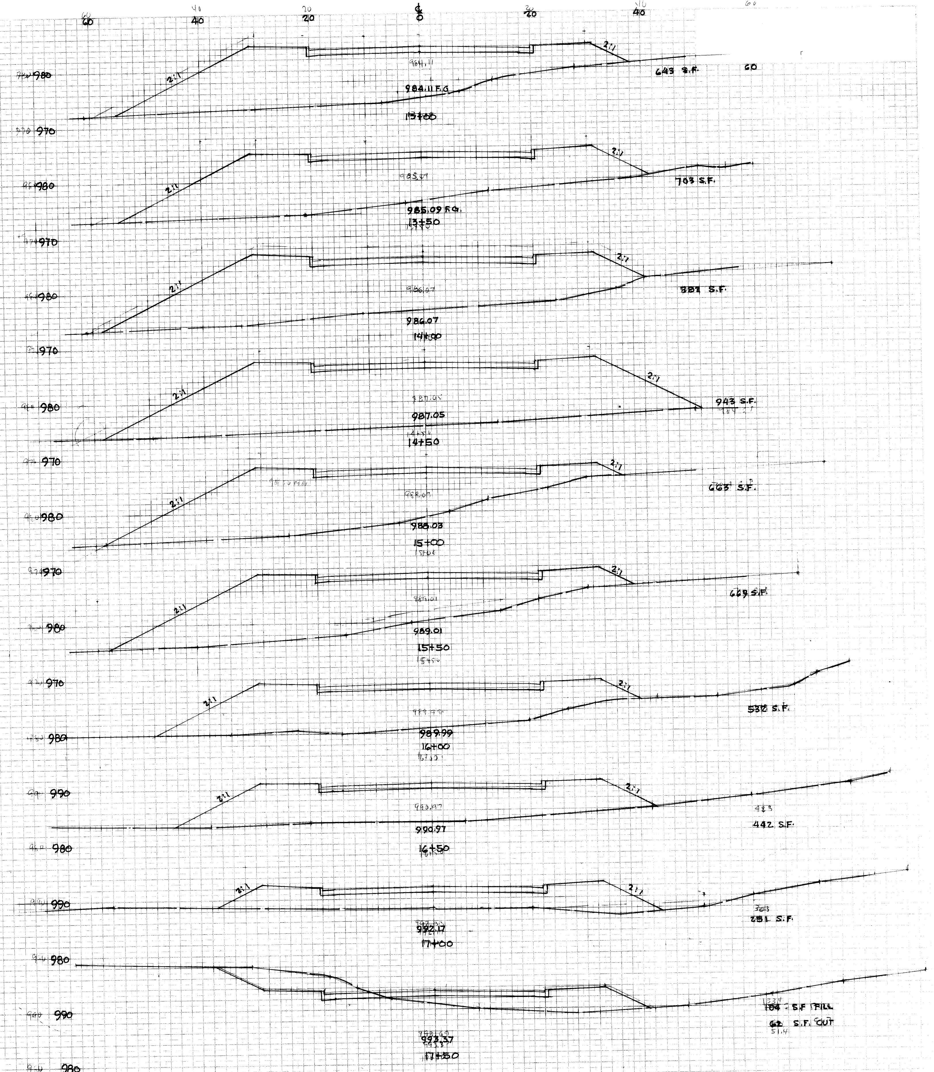
X-SECTIONS VARMINGTON RD. S.E. 8+50 TO 17+50
