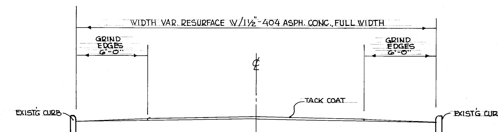
TYPICAL SECTION SCALE 1" = 5'
