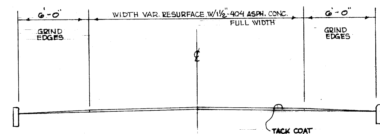
TYPICAL SECTION SCALE 1"=5'
