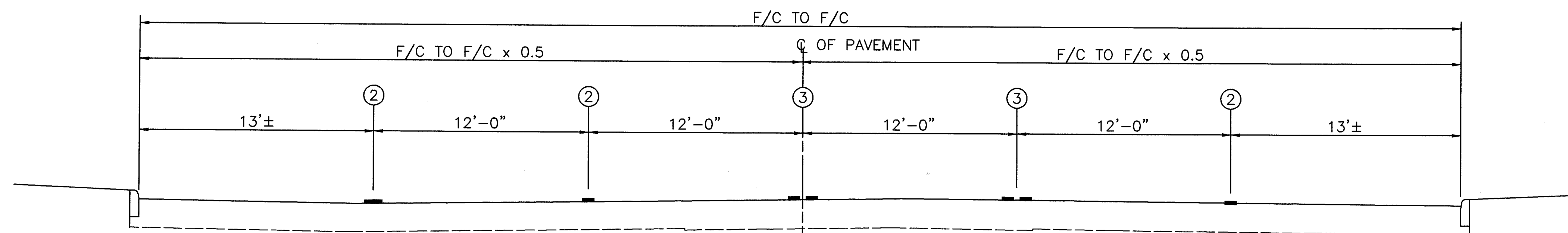
PROPOSED PAVEMENT MARKINGS TYPICAL SECTION - 6-LANE LINCOLN WAY EAST
