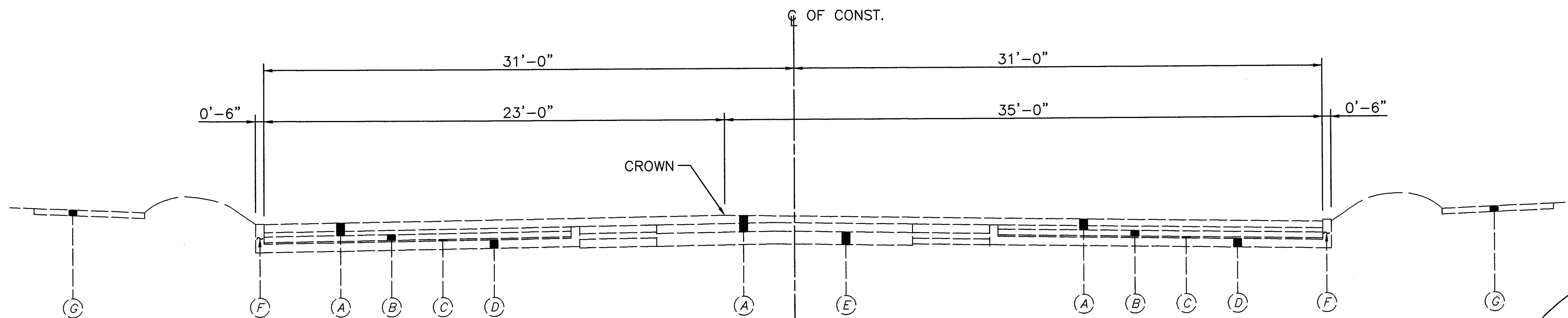
EXISTING TYPICAL SECTION
