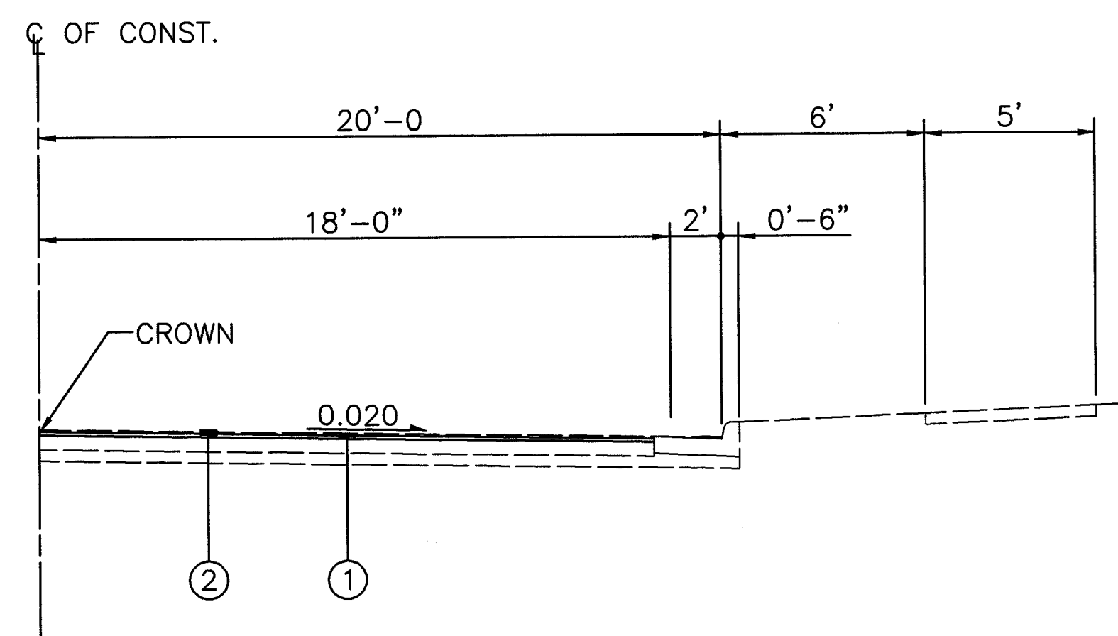
PROPOSED RESURFACING TYPICAL SECTION - 23rd. STREET N.E. SYMMETRICAL
