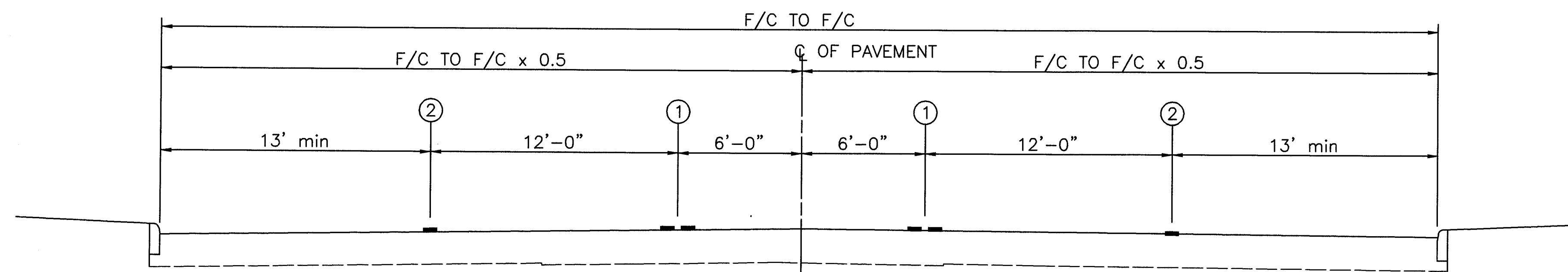
PROPOSED PAVEMENT MARKINGS TYPICAL SECTION - 5-LANE LINCOLN WAY EAST
