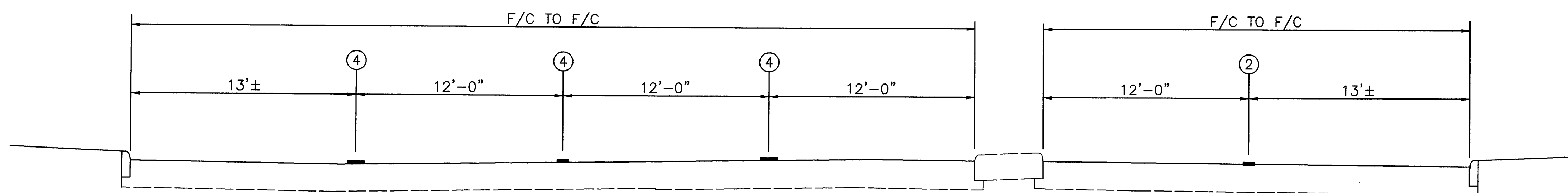
PROPOSED PAVEMENT MARKINGS TYPICAL SECTION - 6-LANE W/ ISLAND LINCOLN WAY EAST
