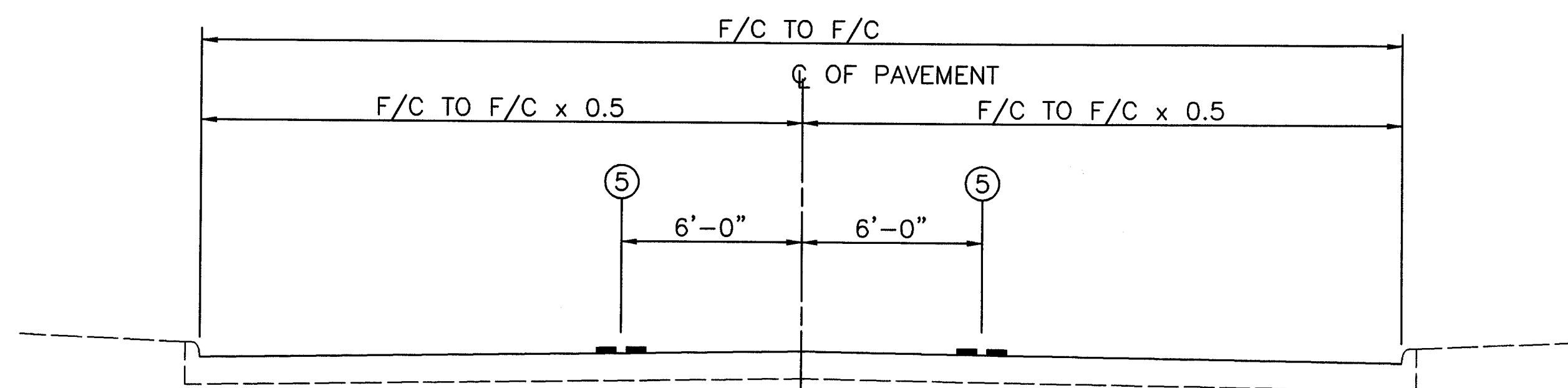
PROPOSED PAVEMENT MARKING TYPICAL SECTION - 3-LANE SIDE ROADWAY
