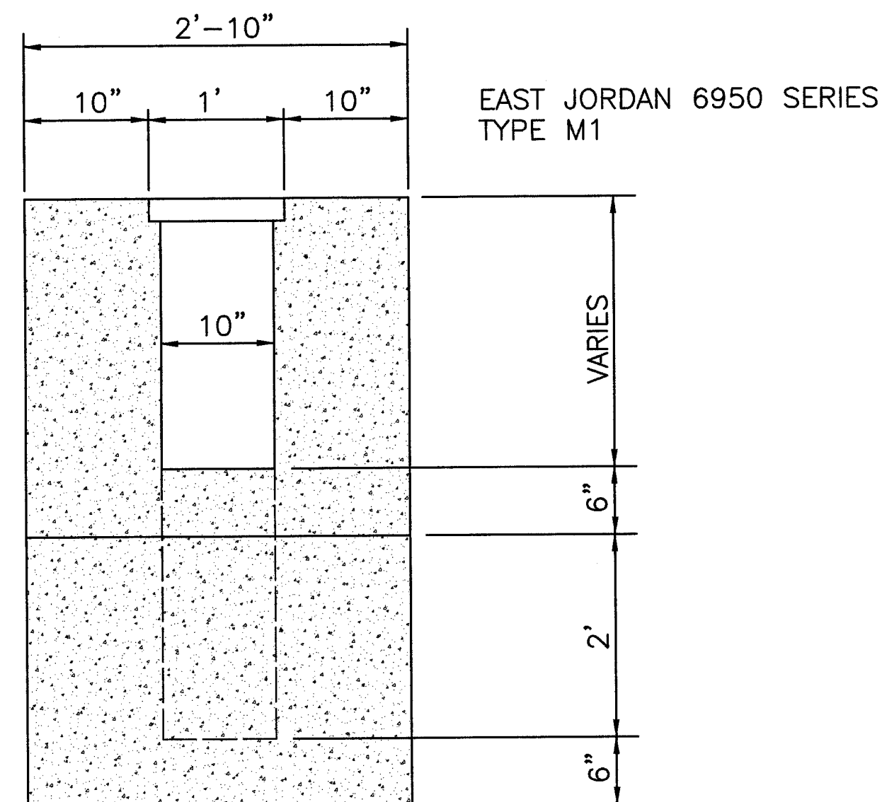
SECTION D-D SCALE: 1=1 (SEE NOTE THIS PAGE)
