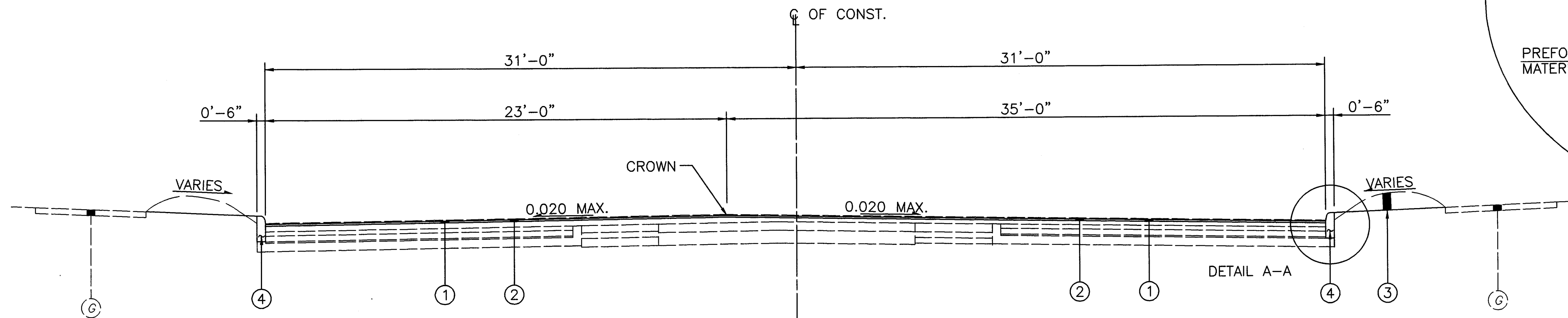
PROPOSED RESURFACING TYPICAL SECTION - LINCOLN WAY EAST
