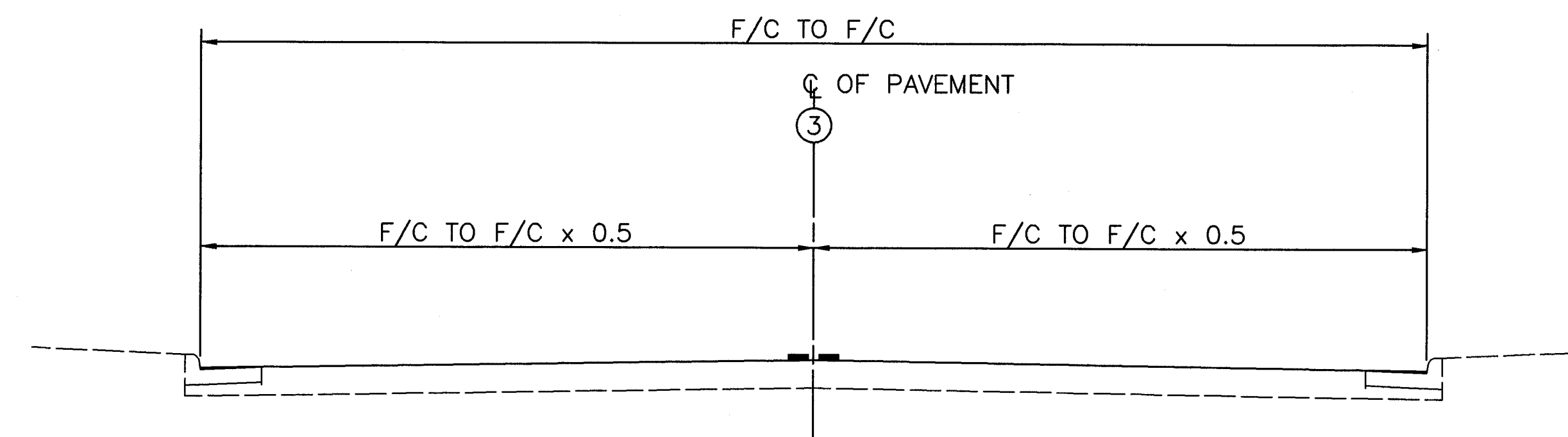
PROPOSED PAVEMENT MARKING TYPICAL SECTION - 2-LANE SIDE ROADWAY
