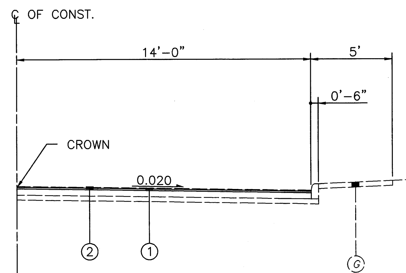
PROPOSED RESURFACING TYPICAL SECTION - 16th. STREET N.E. SYMMETRICAL
