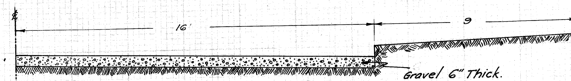
TYPICAL CROSS-SECTION OF ROADWAY
