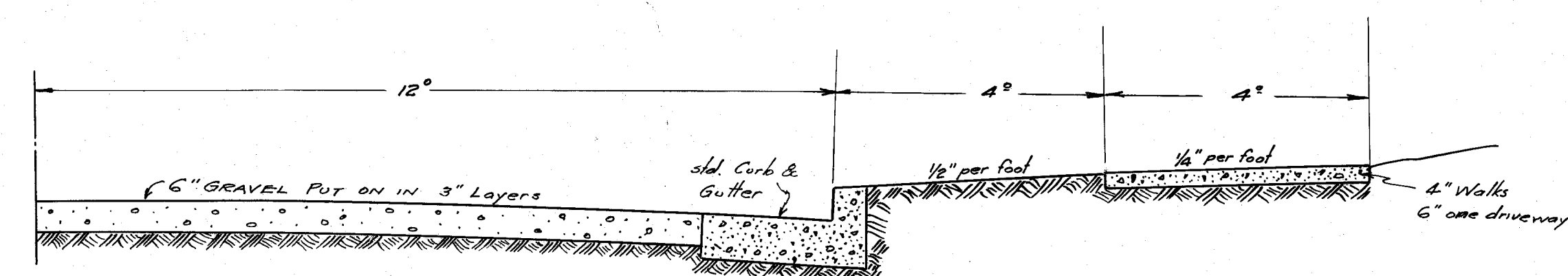
STANDARD SECTION OF ROADWAY
