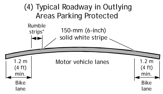
Figure 15-1. Illustrations. Typical bike lane cross sections.
