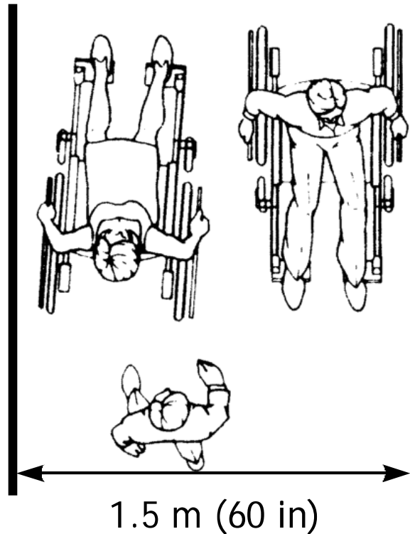
Figure 8-8. Illustration. Minimum passage width for two wheelchairs.
