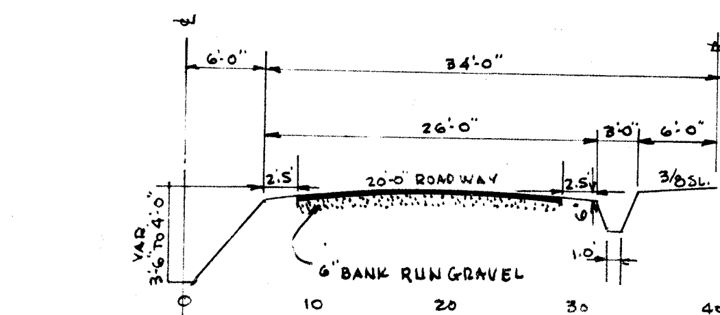
TYPICAL HALF SECTION 80' STREET
