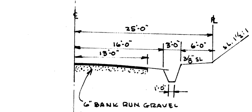
TYPICAL HALF SECTION 50' STREET
