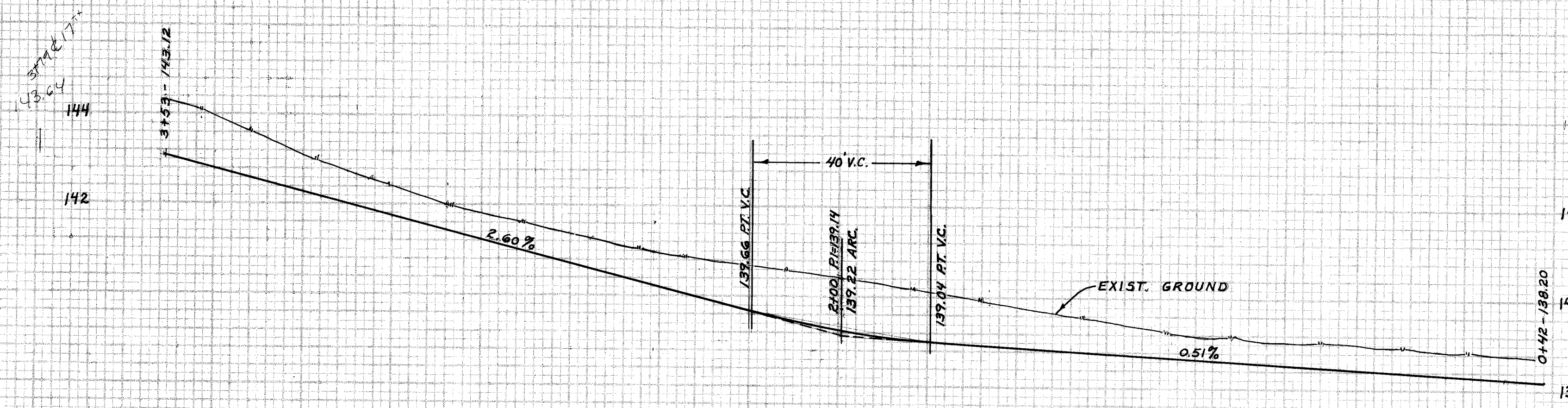
PROFILE AUBURN AVE. N.W. WEST OF 15 TH ST. N.W.
