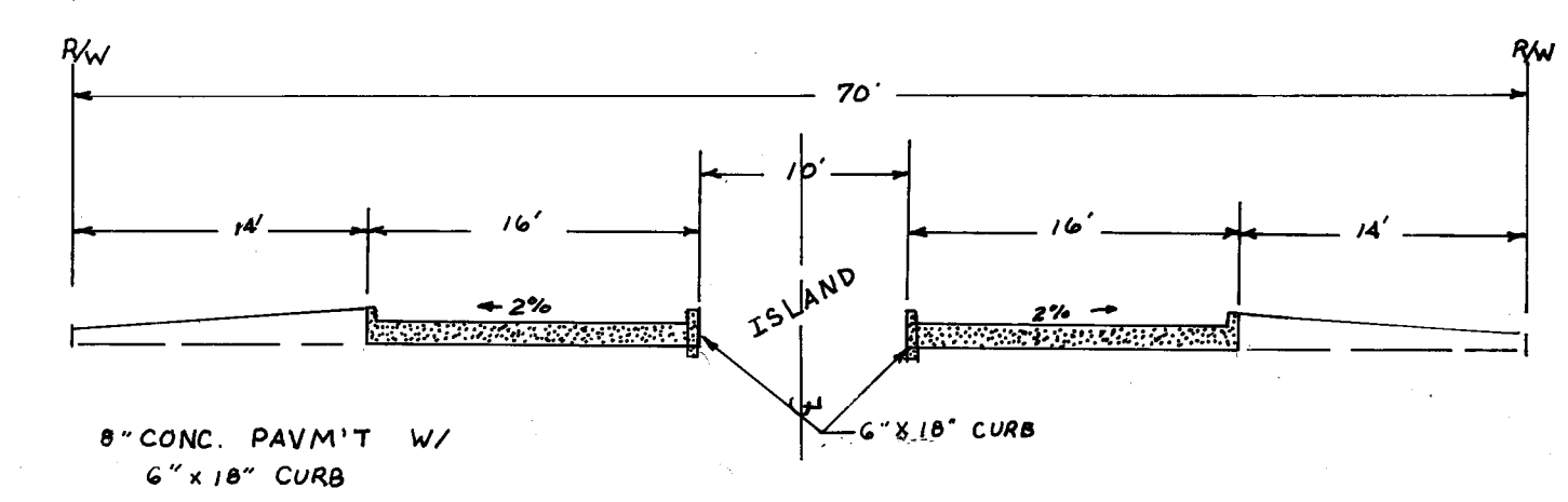
TYPICAL SEC. SCALE 1" = 10'
