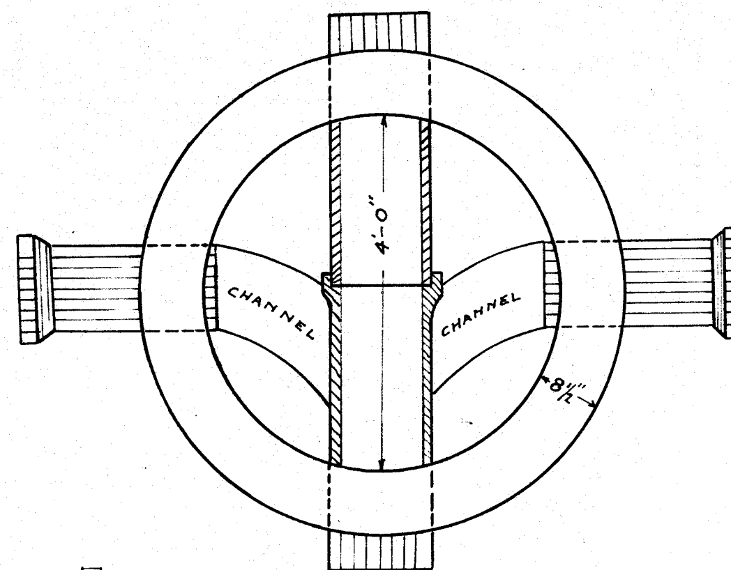
PLAN OF DROP MANHOLE FOR SANITARY SEWER. BRICK CONSTRUCTION.
