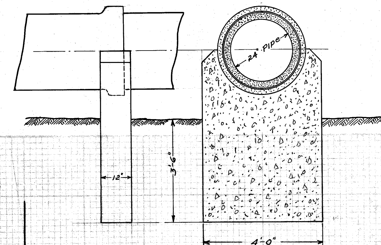
DETAIL OF PIPE CHAIRS Scale 1" = 20' Concrete Mix - 4 1/2 SKS cement to each cubic yd. of finished work.
