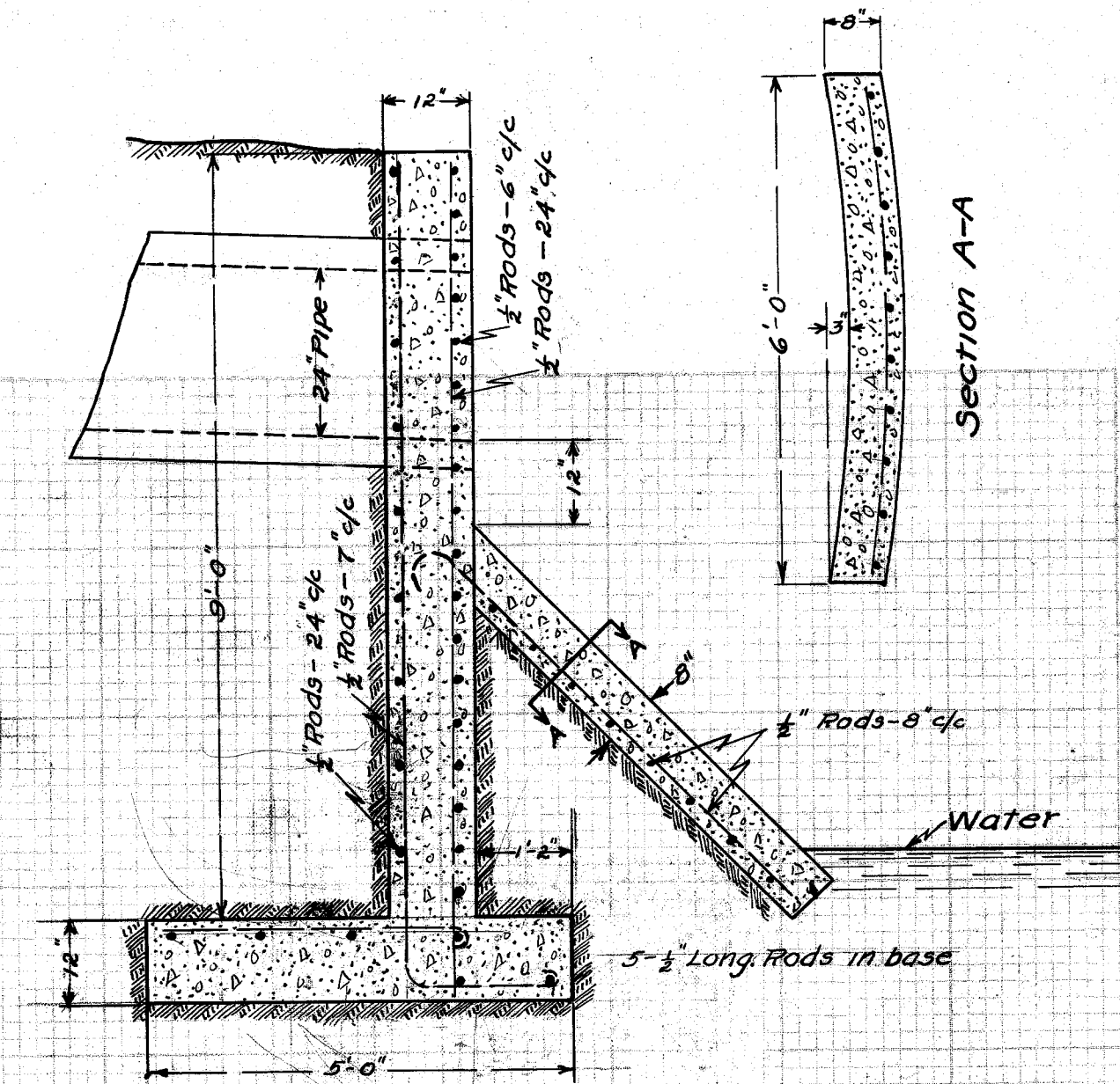
DETAIL OF WALL AT OUTFALL Scale 1" = 20' Length of Wall = 7 ft. Concrete Mix - 6 SKS cement to each cubic yd. of finished work.
