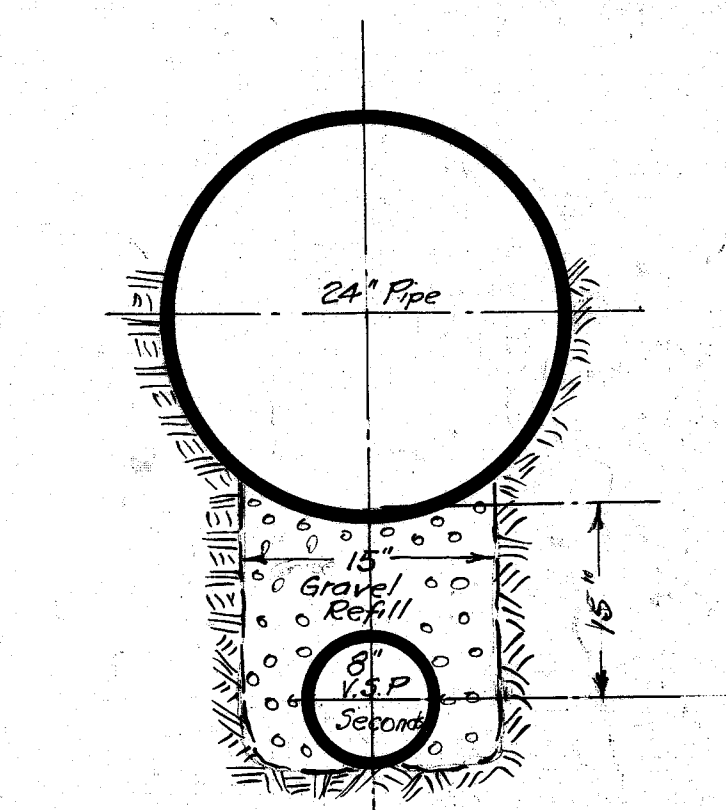
DETAIL OF 8" UNDERDRAIN
