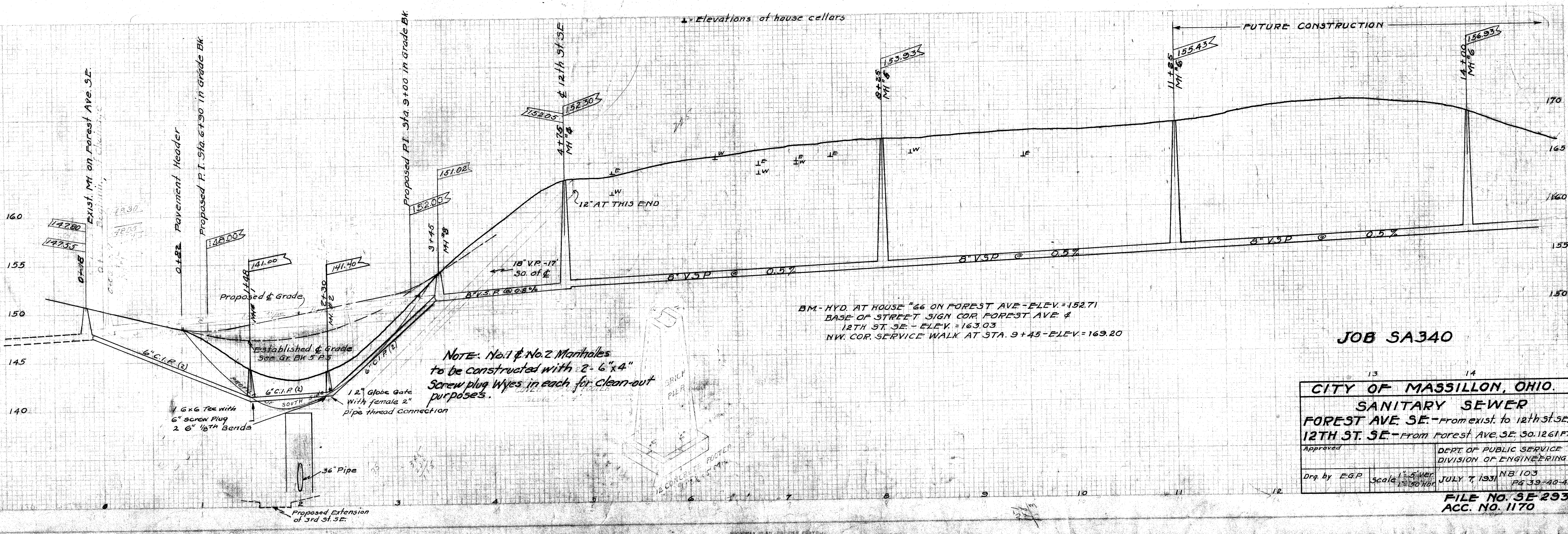
FOREST AVE. SE. 50' PLAN "B"
