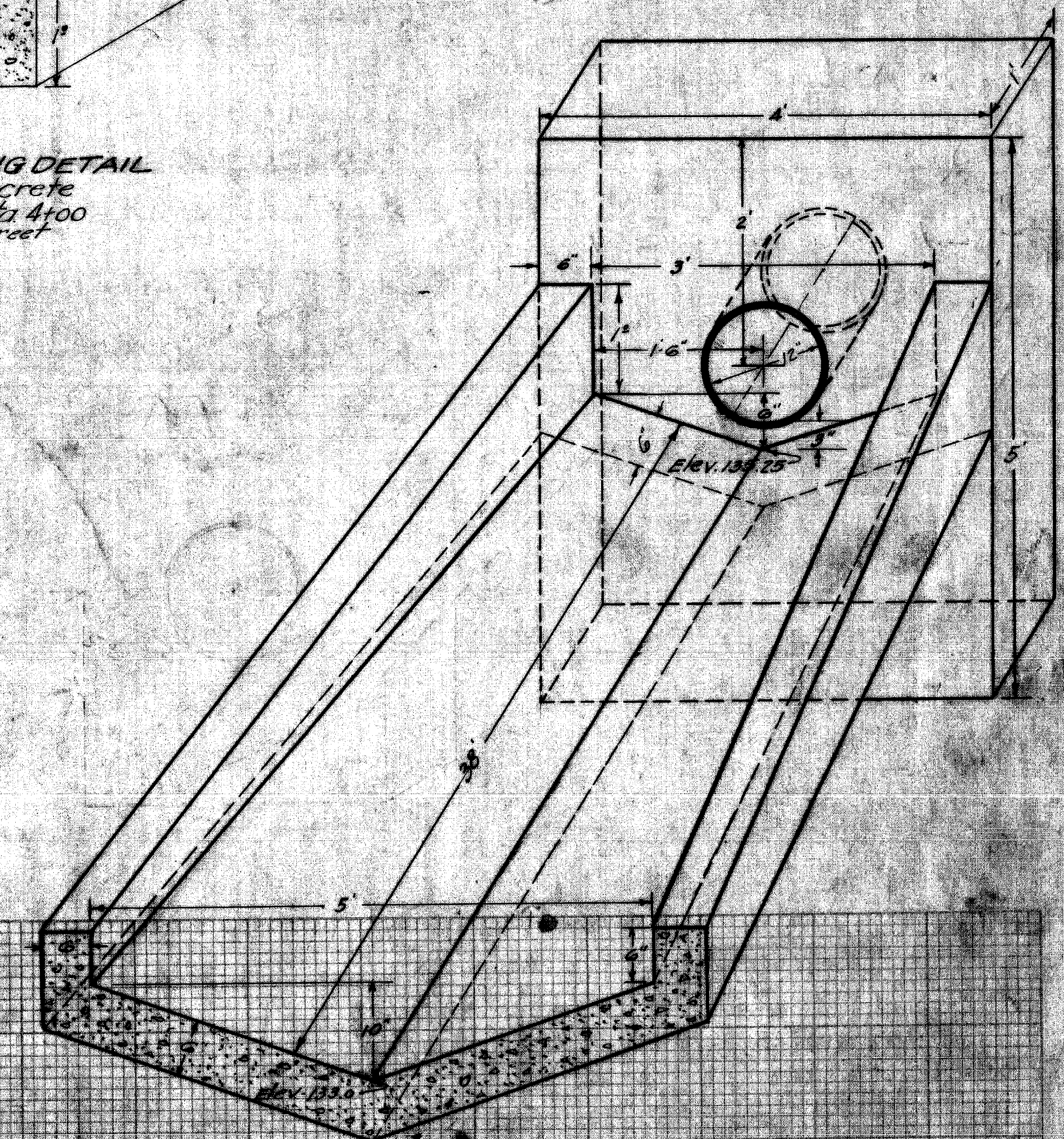
CONCRETE APRON & HEADWALL DETAIL Class 1 Concrete 6 C.Y.
