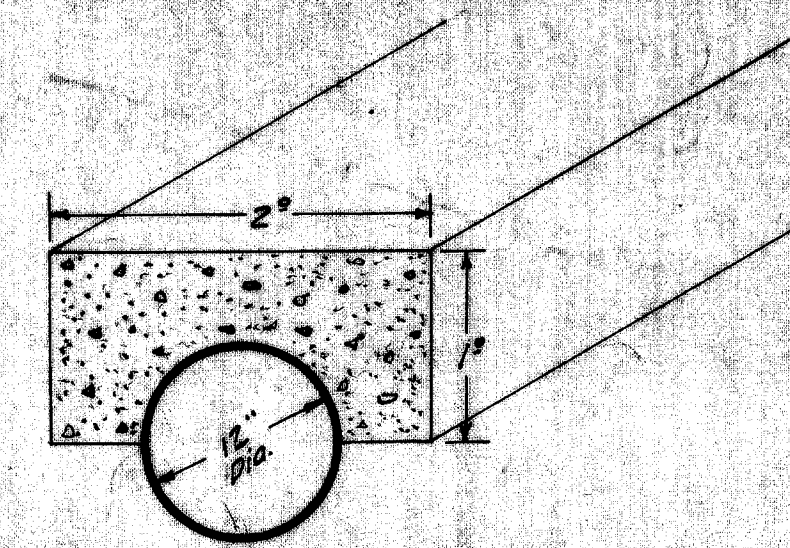
CONCRETE CASING DETAIL Class 2 Concrete Sta. 2+40 to Sta. 4+00 on Seneca Street
