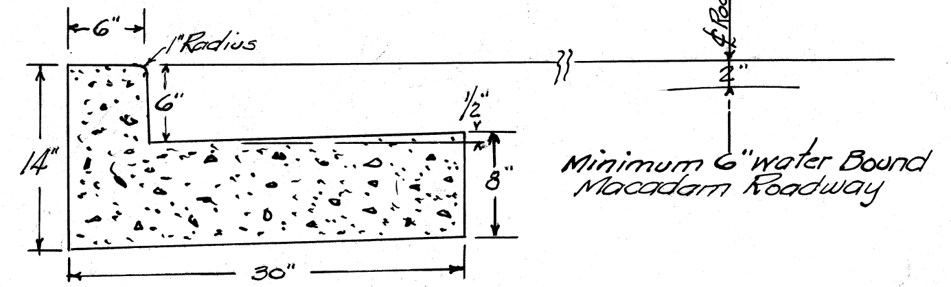
COMBINED CURB & GUTTER DETAIL conc. class 1
