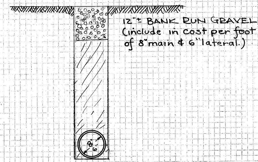
TYPICAL SECTION DITCH
