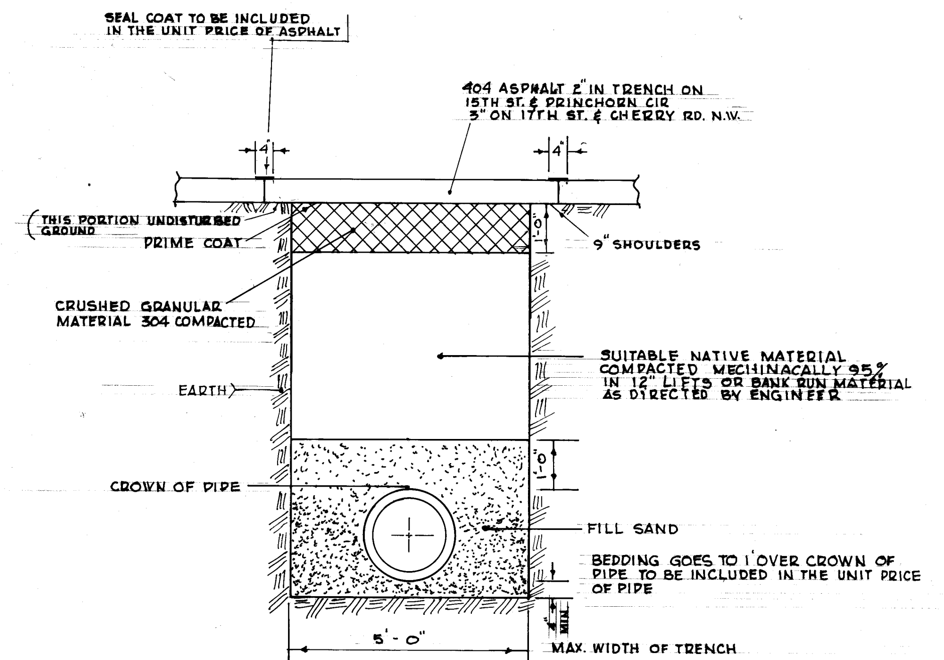
TYPICAL DITCH RESTORATION DETAIL
