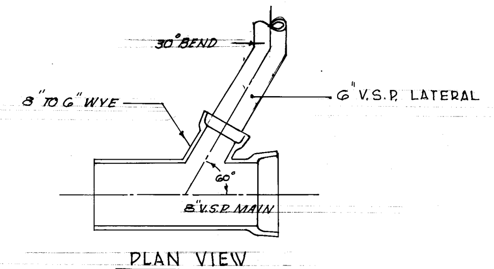
DETAIL OF WYE & LATERAL CONNECTION
