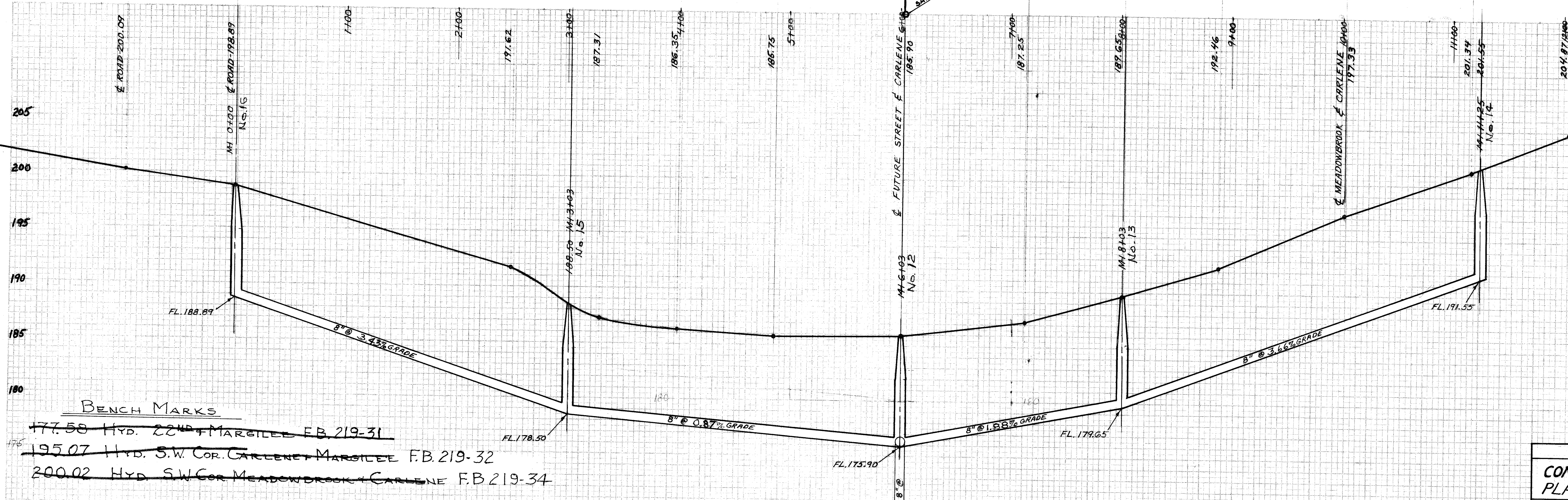
CARLENE AVE. S.W. PROFILE & SEWER
