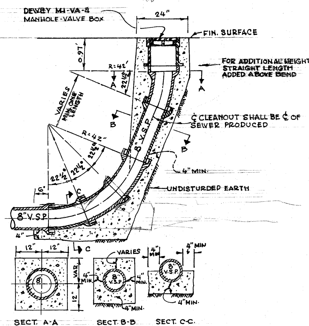
TYPICAL CLEANOUT SCALE 1/2" = 1'-0"
