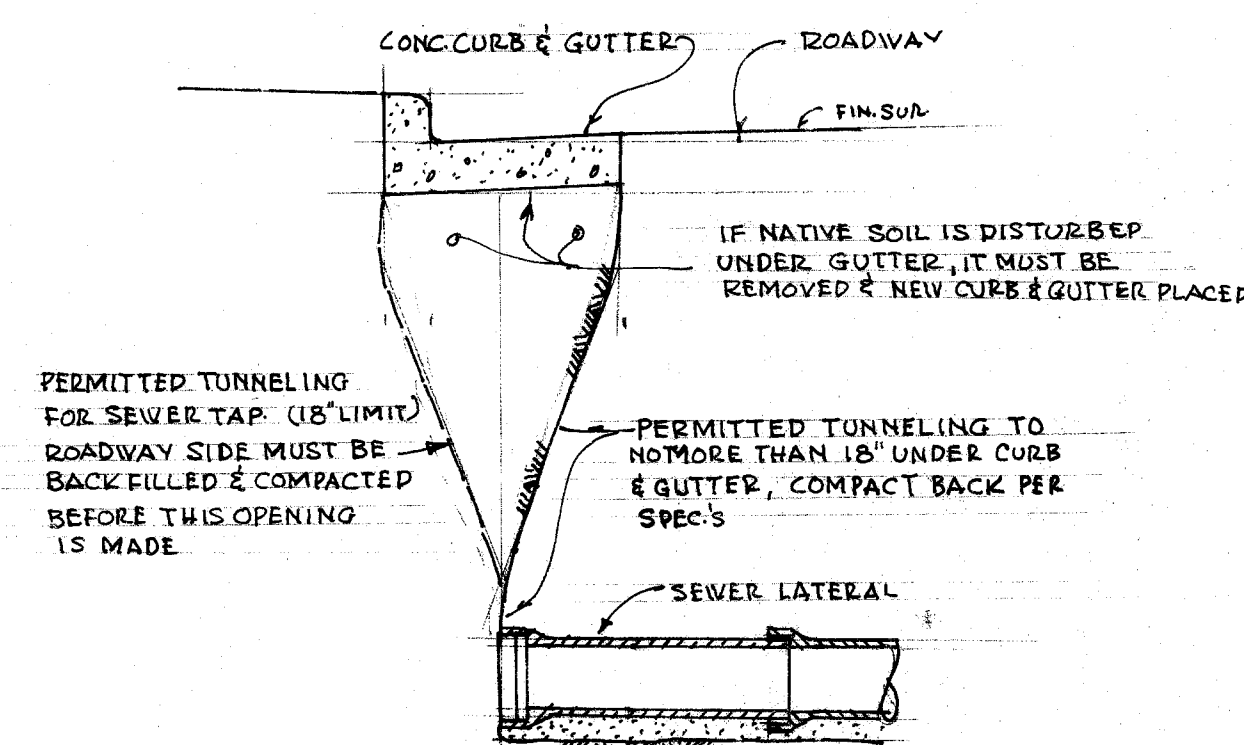
SEWER LATERAL @ EXIST. CURB & GUTTER SCALE 1/2" = 1'-0"
