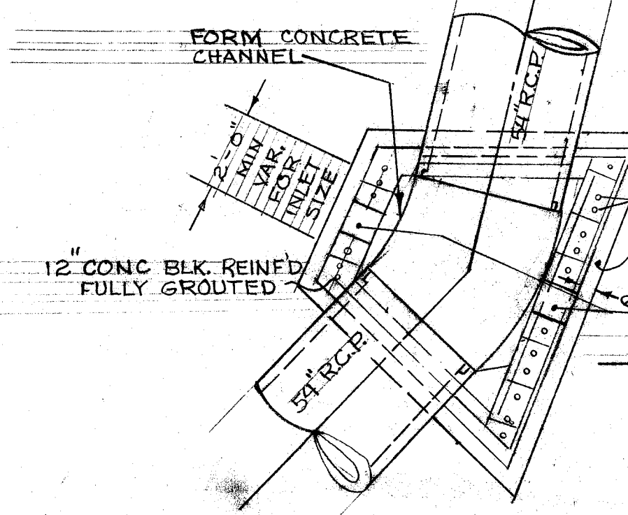
JUNCTION CHAMBER "A" SCALE 1/4" = 1'-0"
