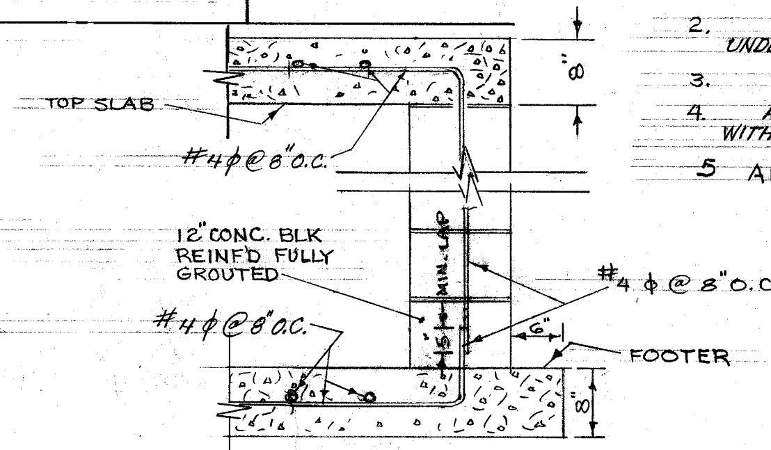
JUNCTION CHAMBER FOOTER DETAIL REINFD SCALE 3/4" = 1'-0"
