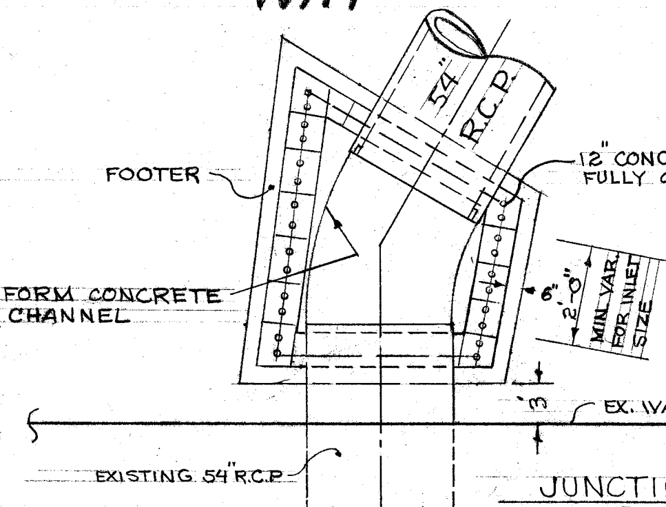
JUNCTION CHAMBER "A" SCALE 1/4" = 1'-0"
