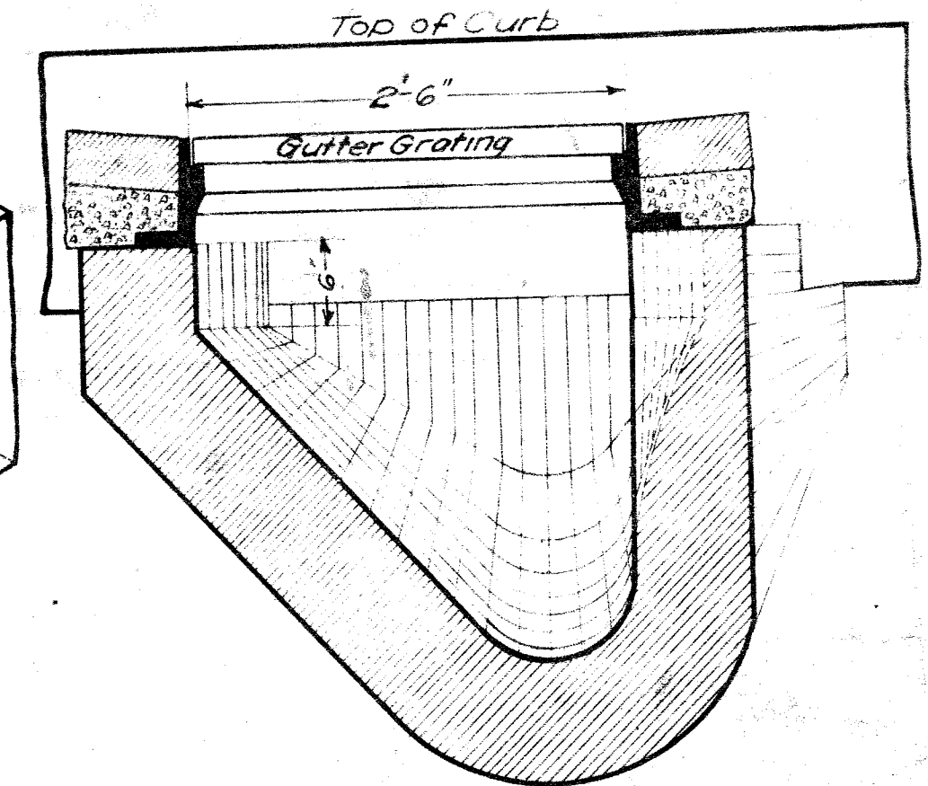
ELEVATION Q-Q FRONT REMOVED
