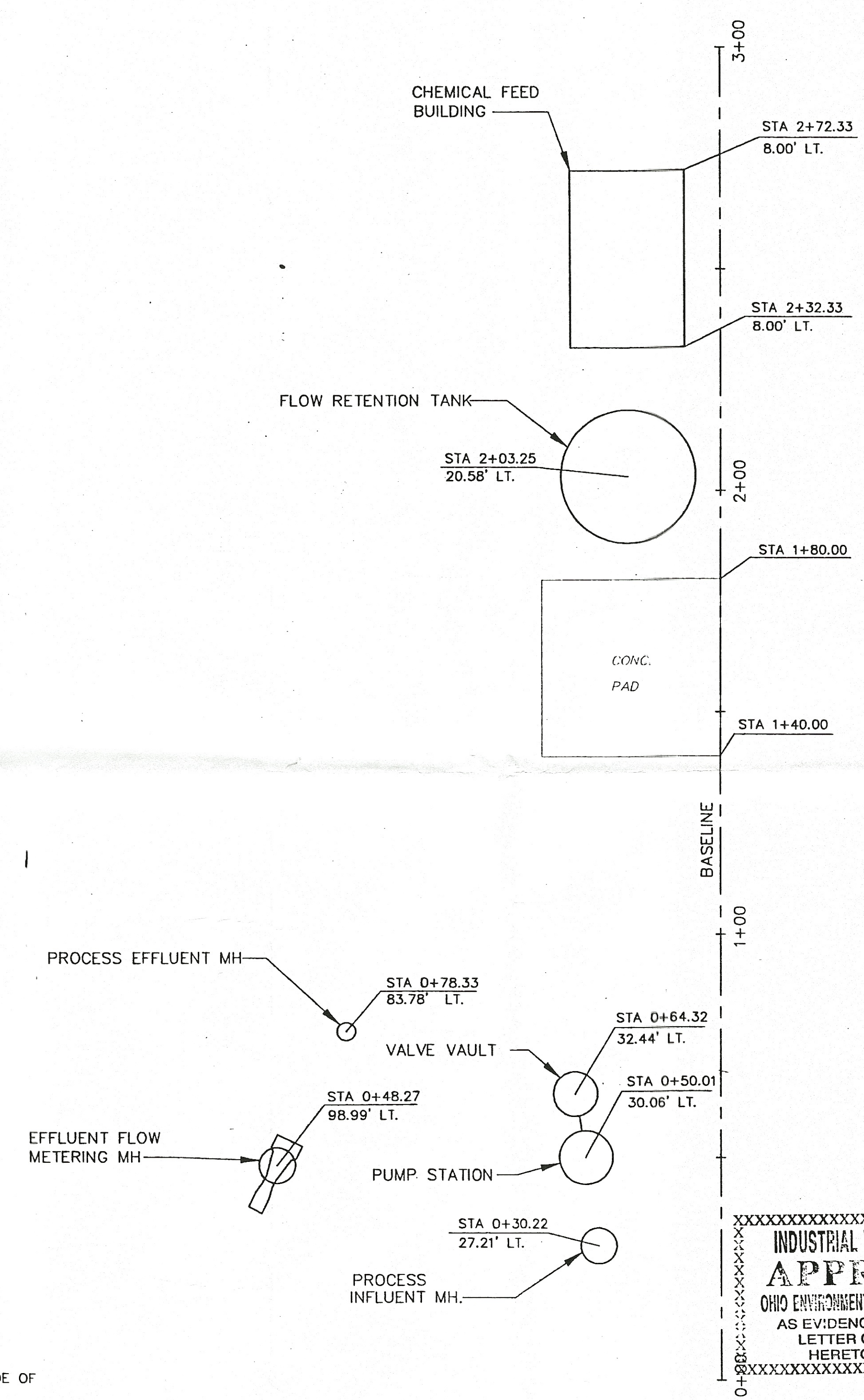
LAYOUT PLAN
