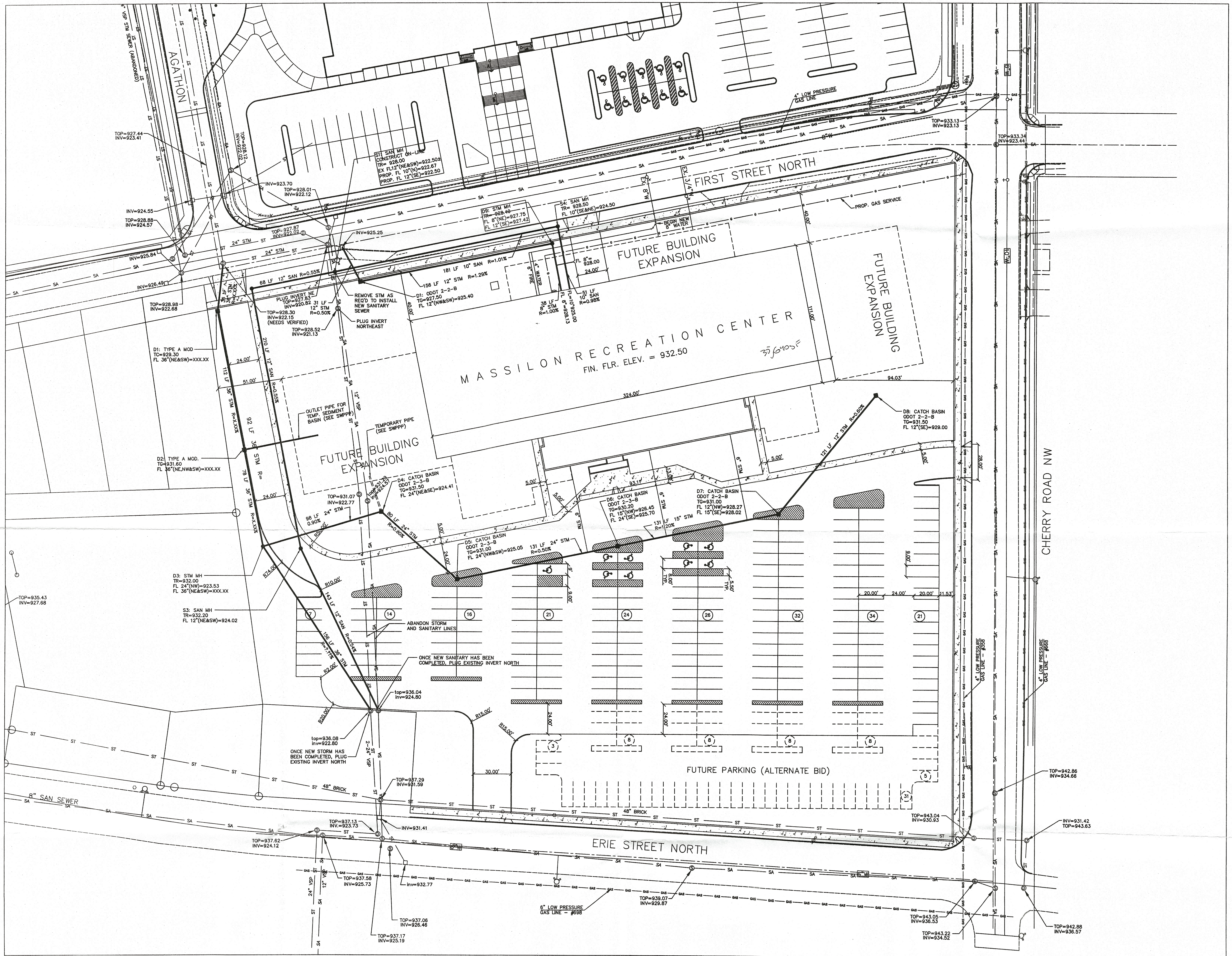
GRADING AND PAVING PLAN 1" = 30'
