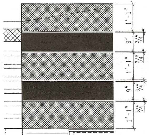
4 ENTRANCE ARCH STRIPING A-4.1 SCALE: 1/2" = 1'-0"
