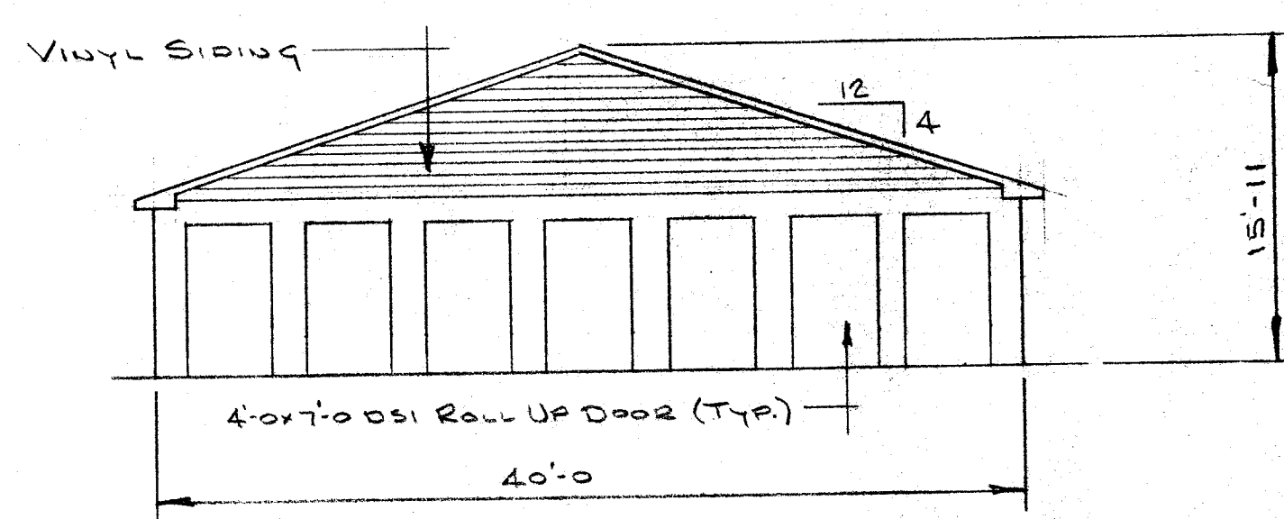
NORTH ELEVATION SCALE: \frac{1}{8}'' = 1'-0''
