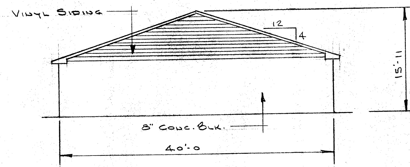
SOUTH ELEVATION SCALE: \frac{1}{8}'' = 1'-0''
