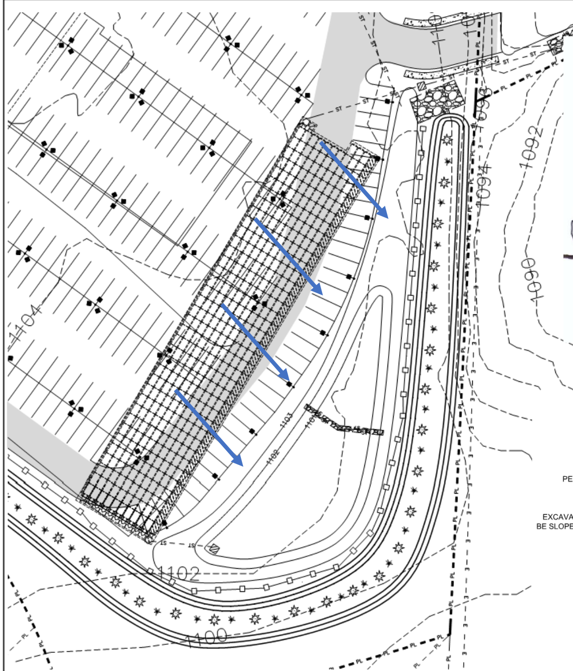
STORMWATER MANAGEMENT PLAN
